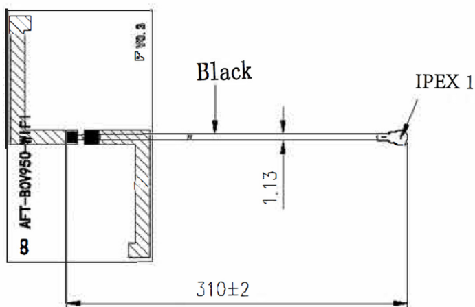
PCB Drawing
