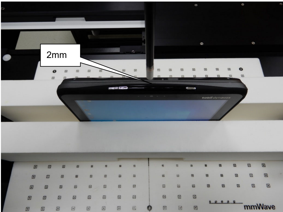
EUT PD_Top_2mm
