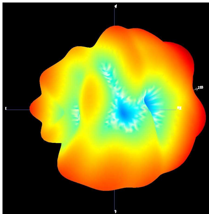
B1.3 3D Pattern for 2500MHz
