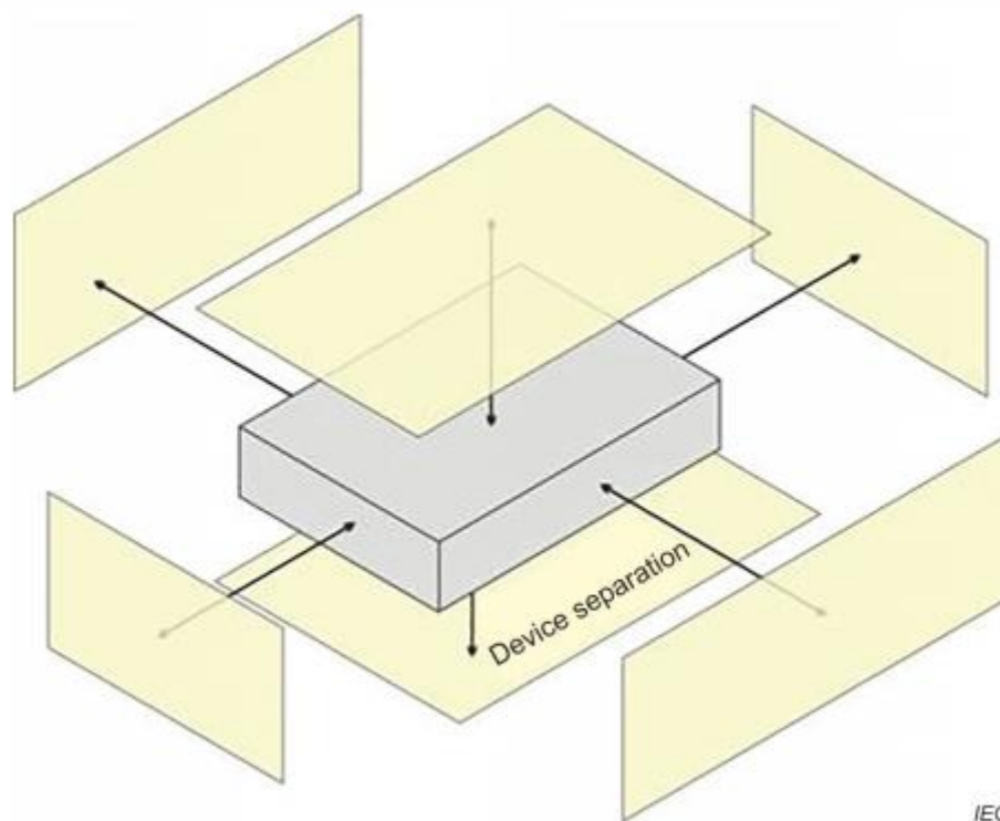
Fig-4.1 Illustration for Tablet Setup
