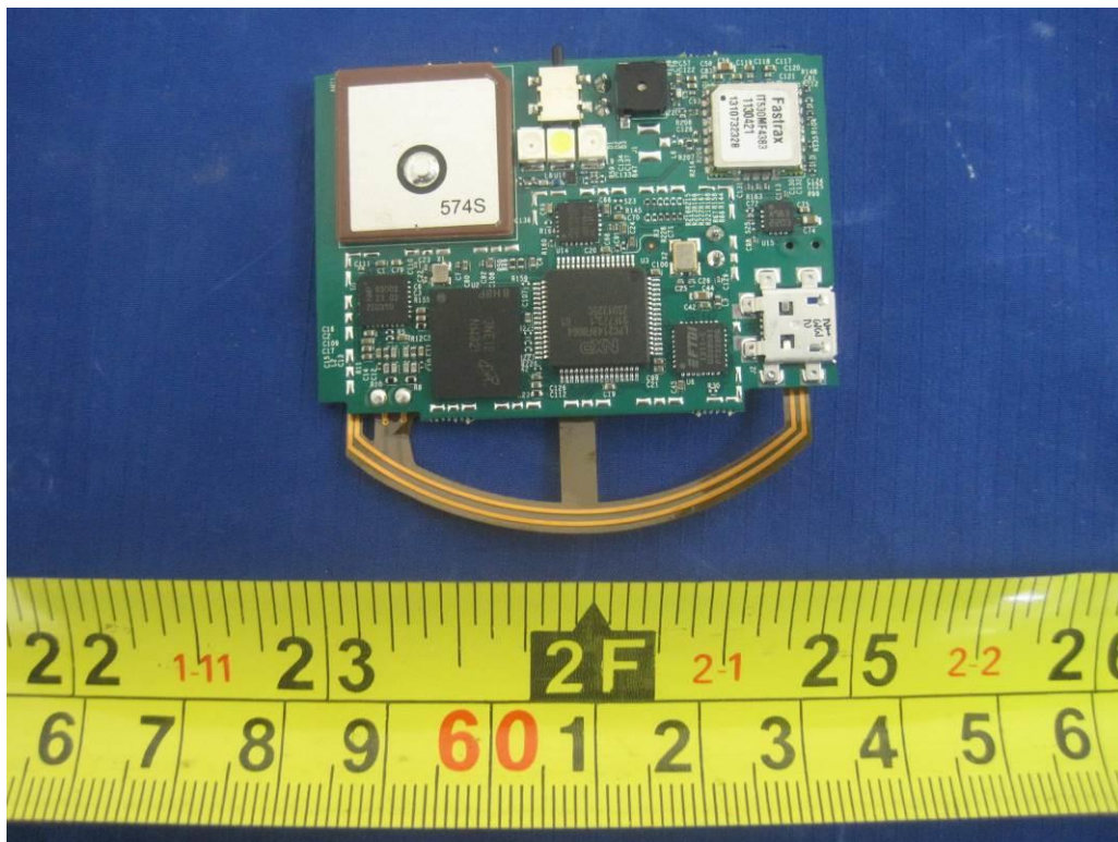
Main Board-Top
