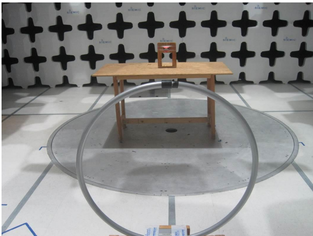
Radiated Emission Test setup (<30MHz) – Front View
