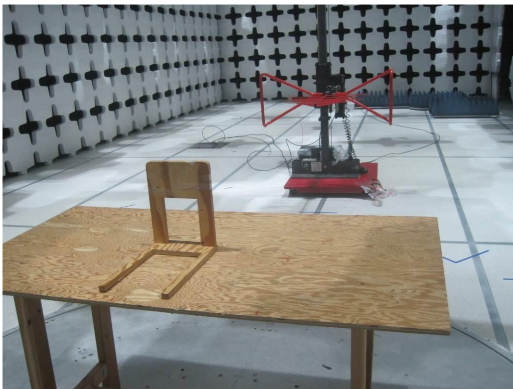
Radiated Emission Test setup (<1GHz) – Rear View
