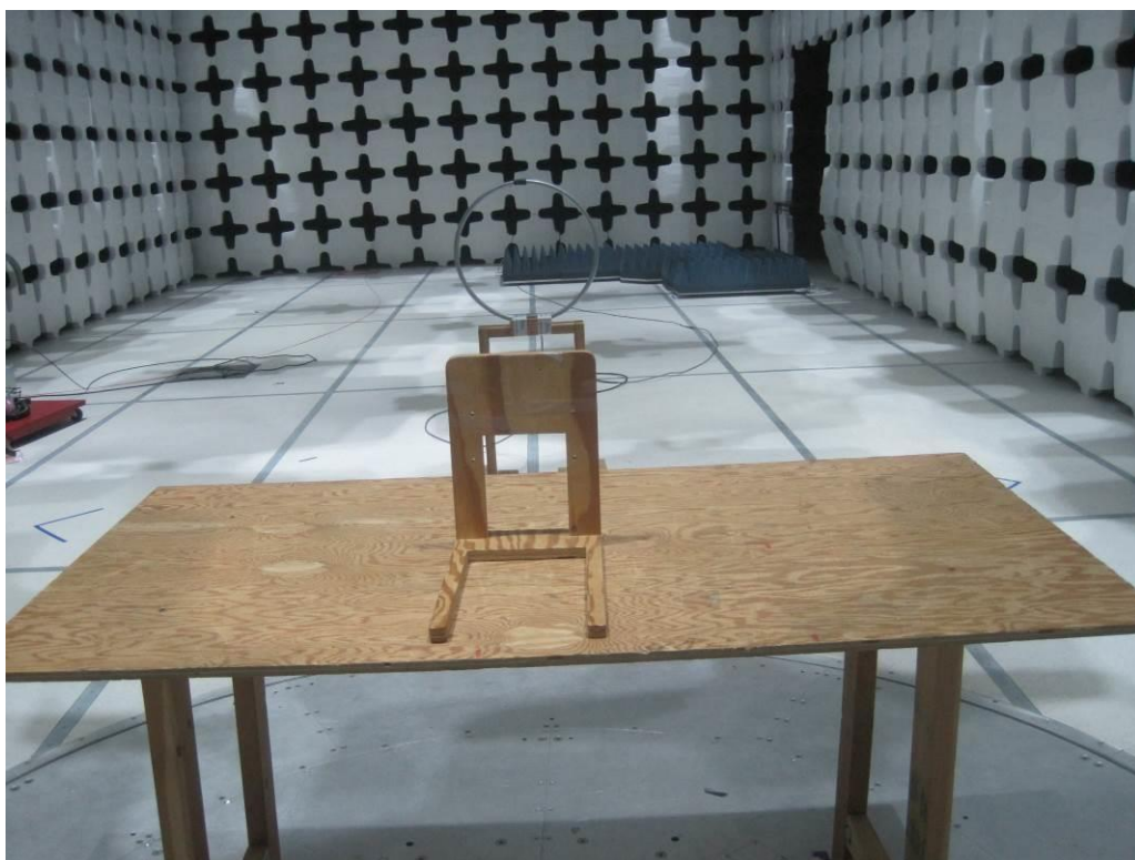
Radiated Emission Test setup (<30MHz) – Rear View
