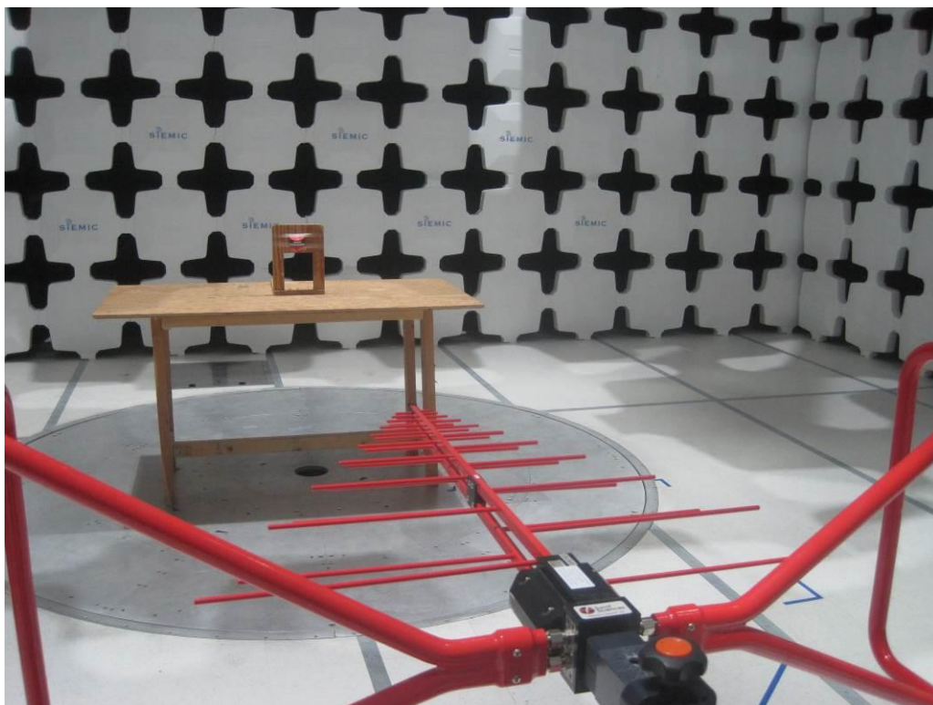
Radiated Emission Test setup (<1GHz) – Front View
