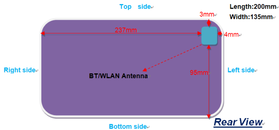
Figure 2: The antenna positions of the DUT
