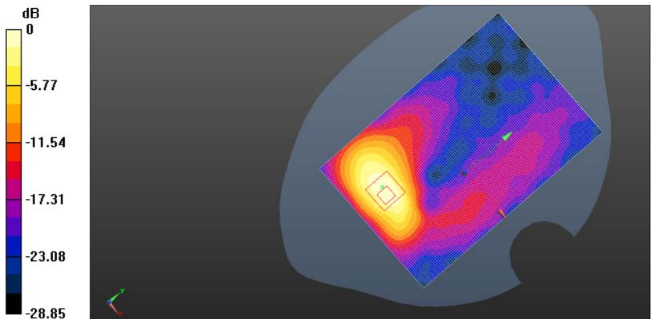
Plot 1: WLAN2450 Rear Side Middle Channel -Channel 1-2412MHz (1Mbps)
