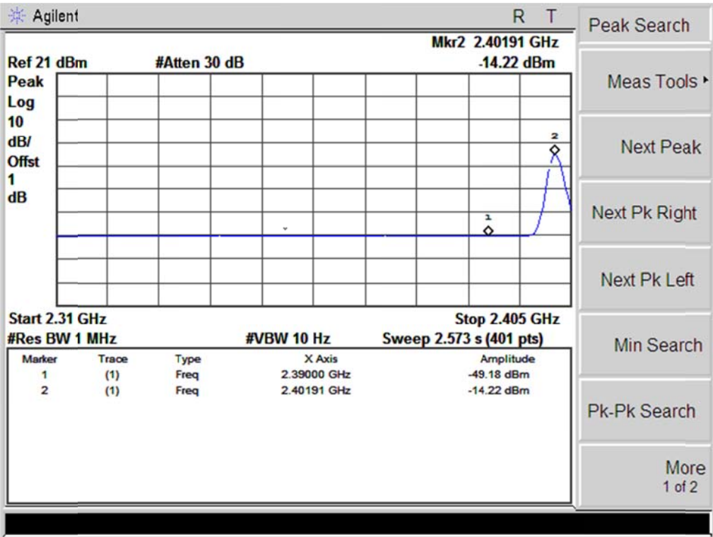
(Plot 4.5.3 A2:Channel 1: 2402MHz)
