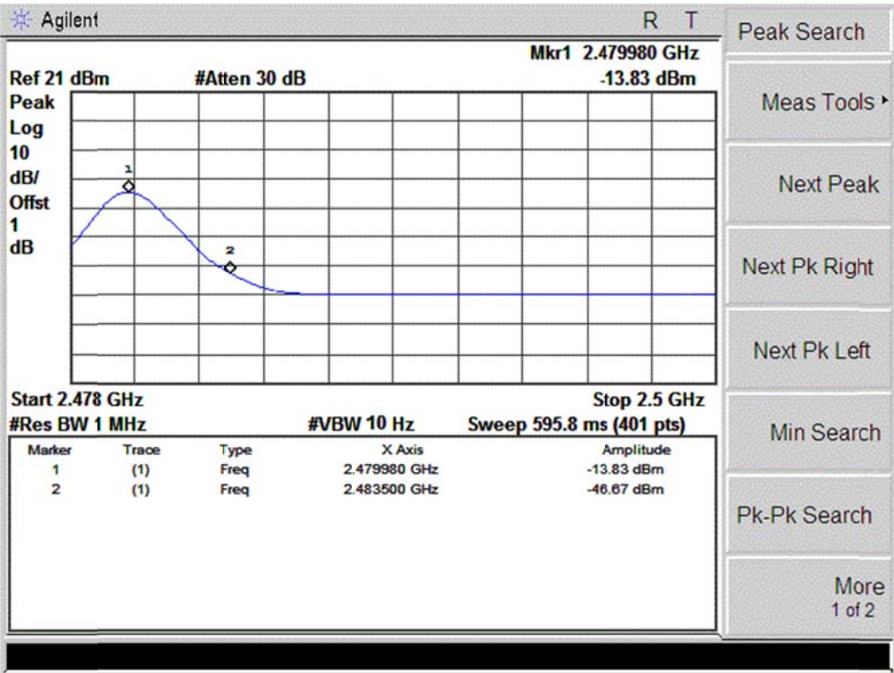
(Plot 4.5.3 A4:Channel 40: 2480MHz)
