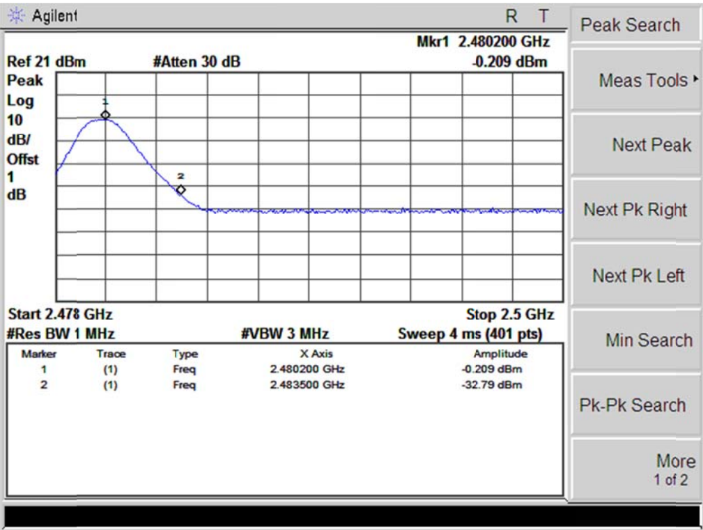
(Plot 4.5.3 A3:Channel 40: 2480MHz)
