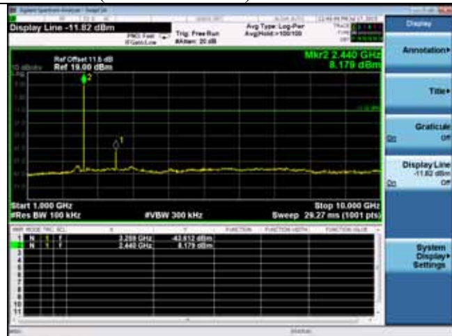
2441MHz(1GHz – 10GHz)
