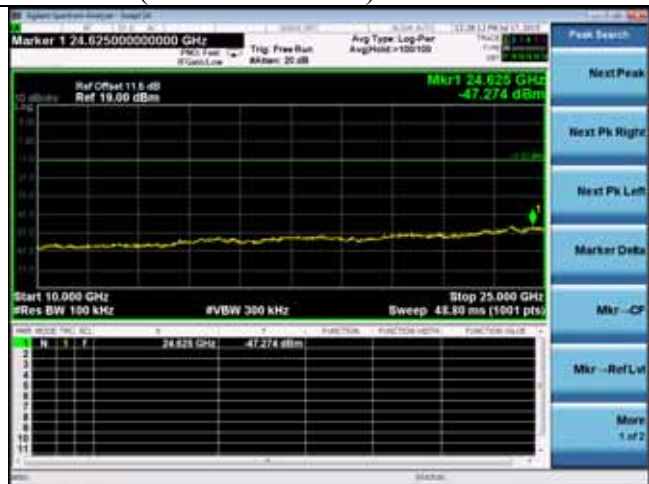
2402MHz(10GHz – 25GHz)
