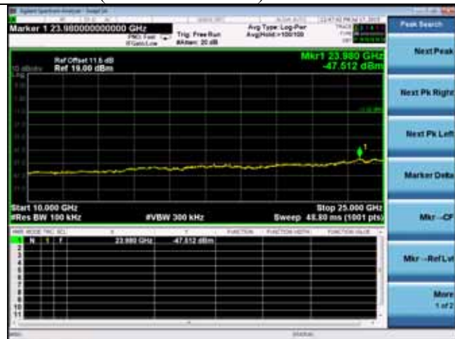
2441MHz(10GHz – 25GHz)
