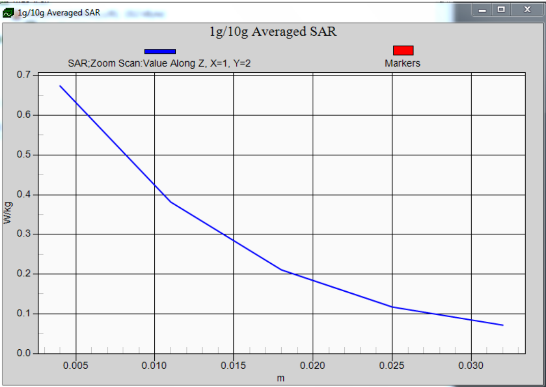
Plot 1: Rear Side (WLAN2450-Middle Channel-Channel 6-2437MHz(1Mbps))
