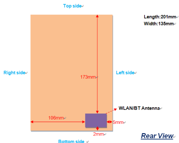
Figure 2: The antenna positions of the DUT
