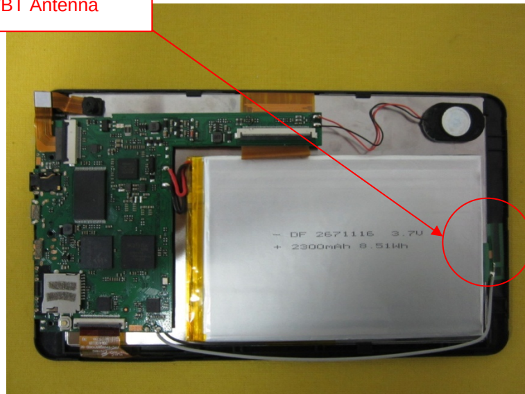
WIFI/BT Antenna
