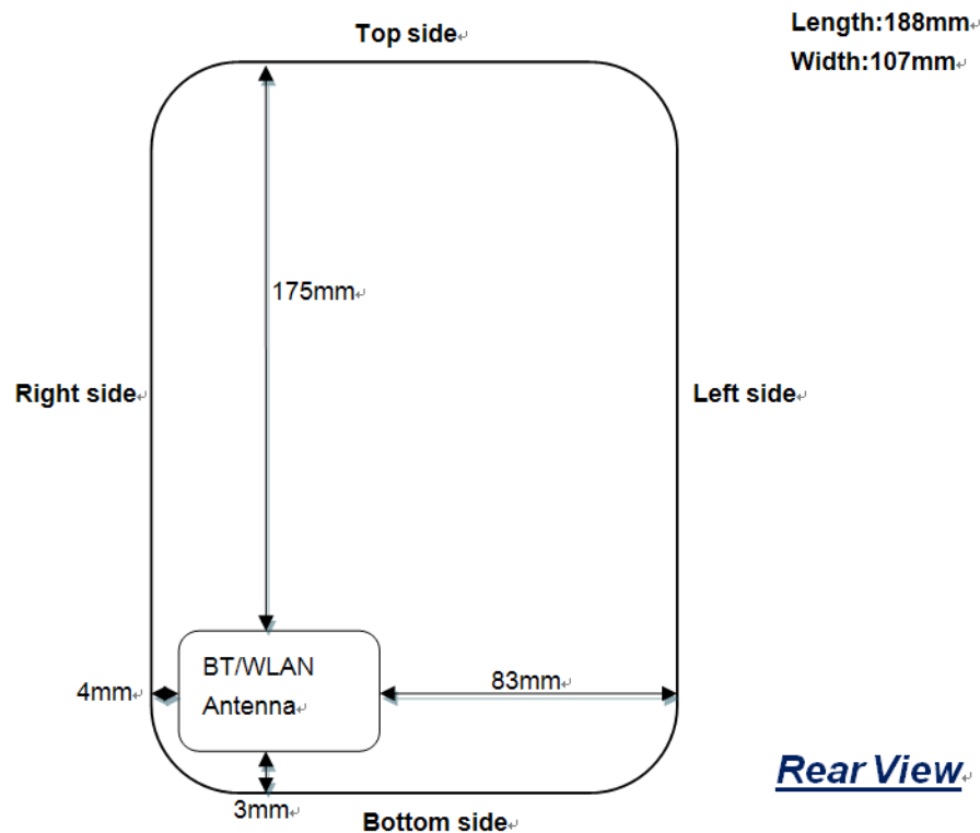
Figure 2: The antenna positions of the DUT
