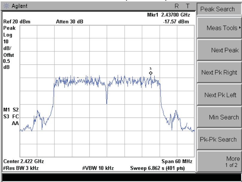
Channel 03 (2422MHz)
