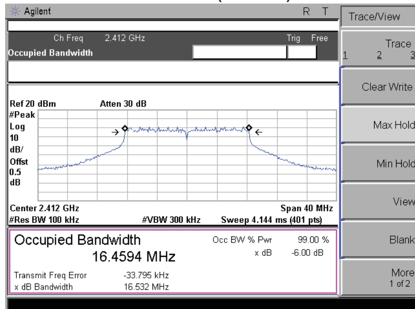
Channel 01 (2412MHz)
