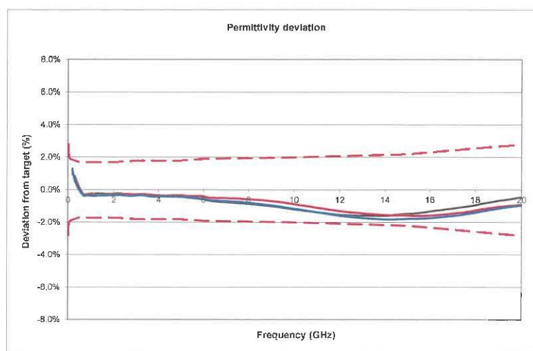
Fig. 4.1 HBBL permittivity deviation from target, 200 MHz – 20 GHz
