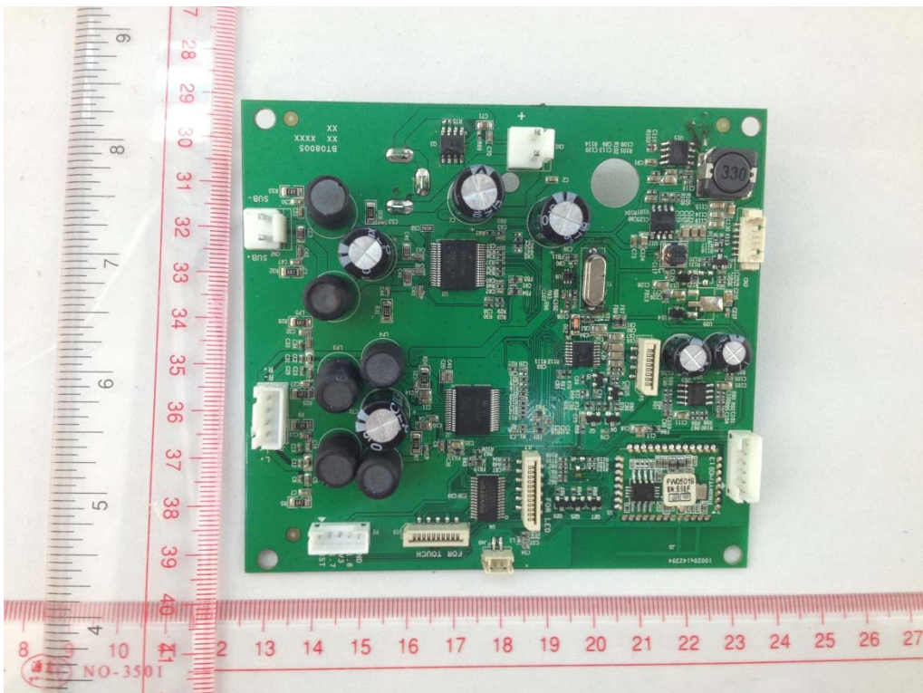
Main Board
