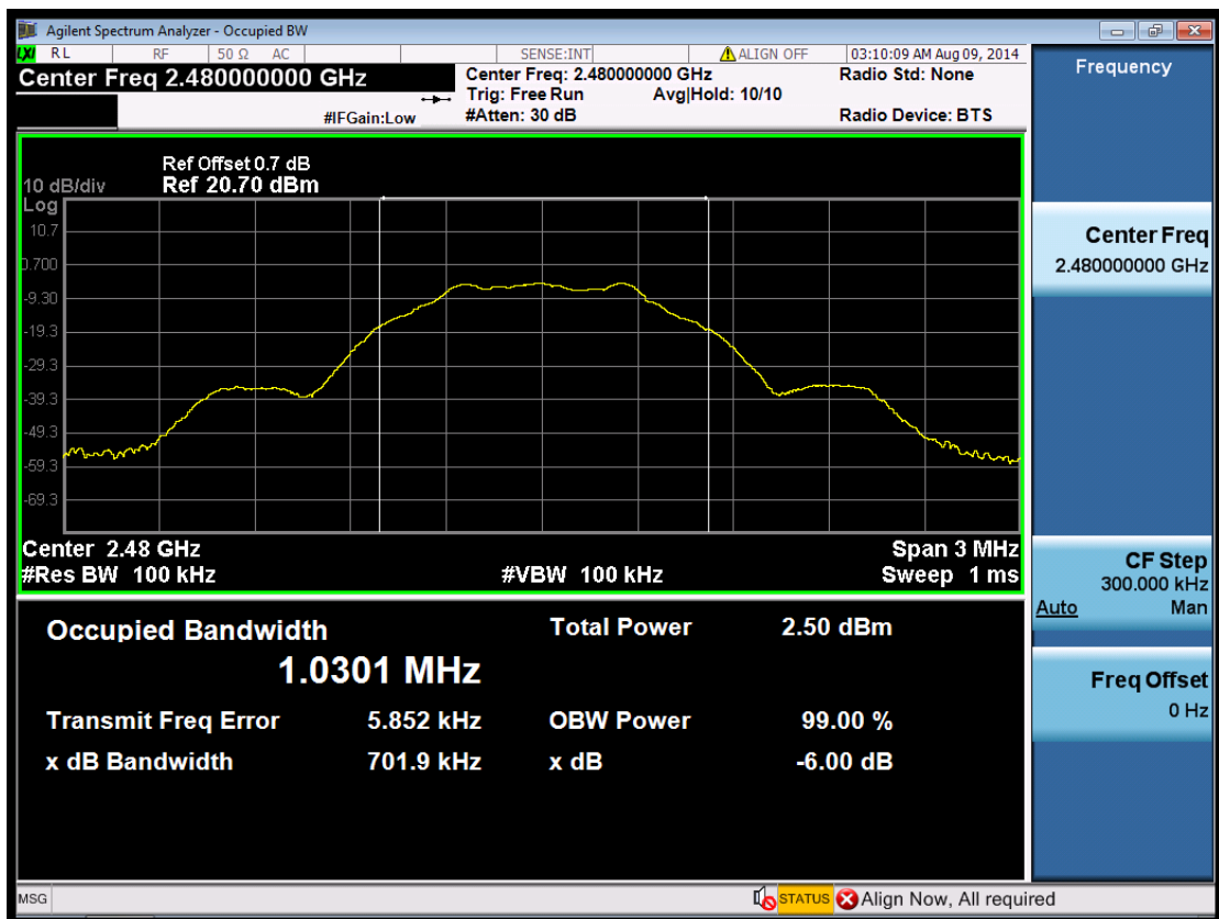
Channel 139: 2480 MHz @ GFSK
