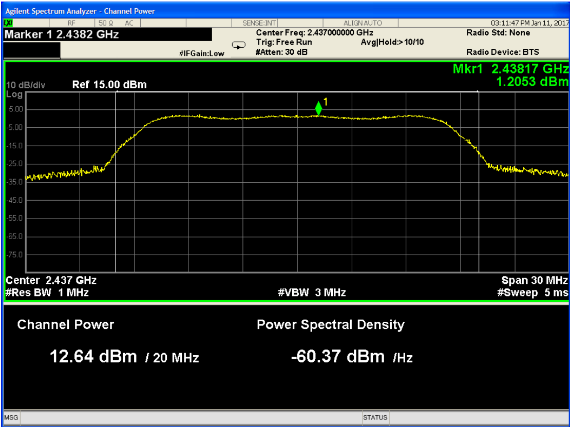
Channel 6: 2.437GHz:
