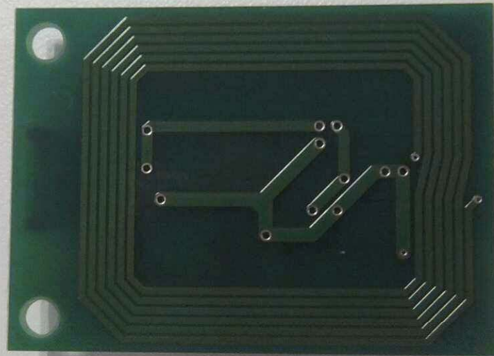
Antenna (Back of the board)
