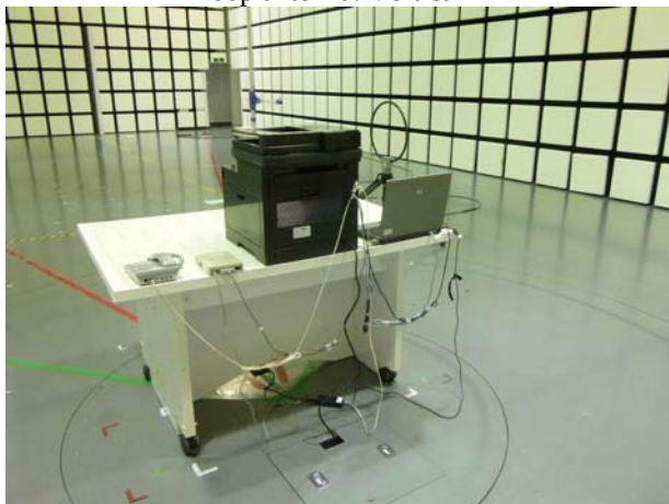
Rear (9 kHz - 30 MHz) Loop antenna: Vertical
