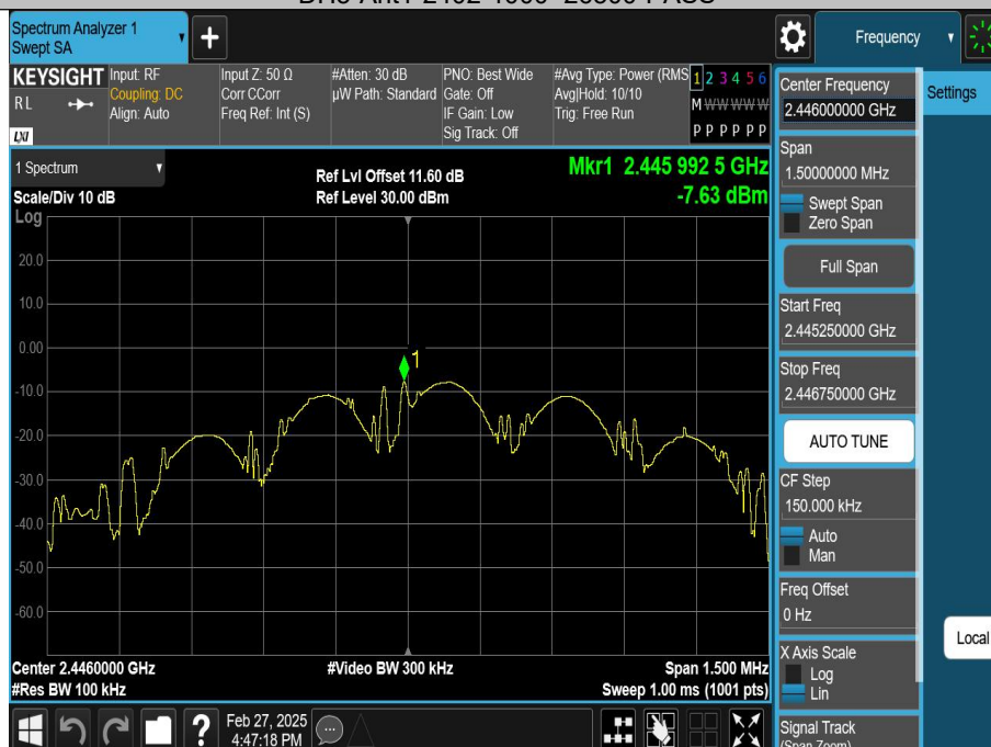
DH5-Ant1-2446-0~Reference-PASS
