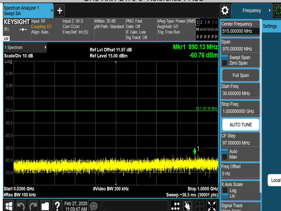
DH5-Ant1-2479-30~1000-PASS
