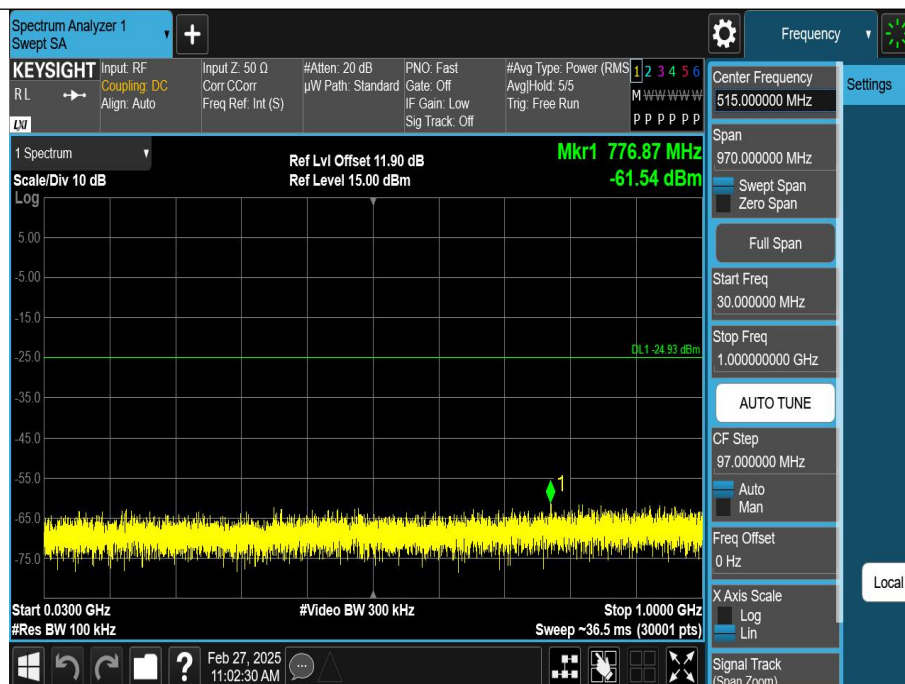
DH5-Ant1-2446-30~1000-PASS
