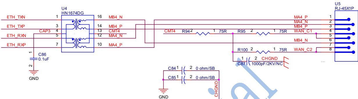
Figure 2-4 The reference design of Ethernet
