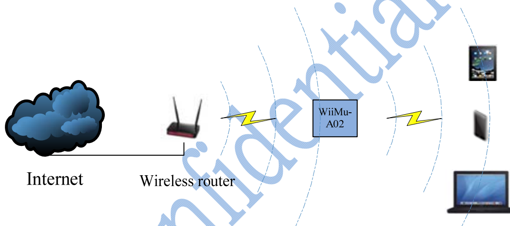
Figure 3-1 WiFiAudio-A28 AP Client mode
