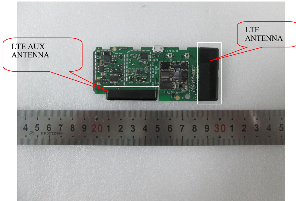
EUT – Main Board Top Shield off View
