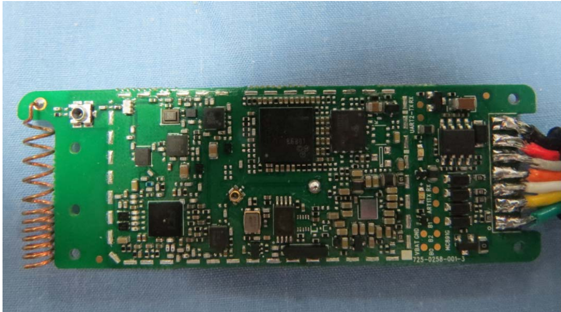
Without Shielding Case-- front side
