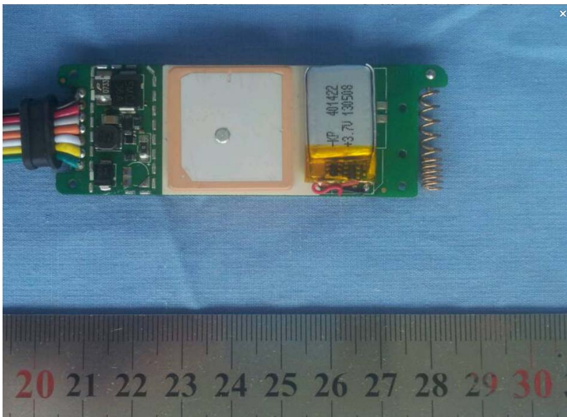
Without Shielding Case --back side
