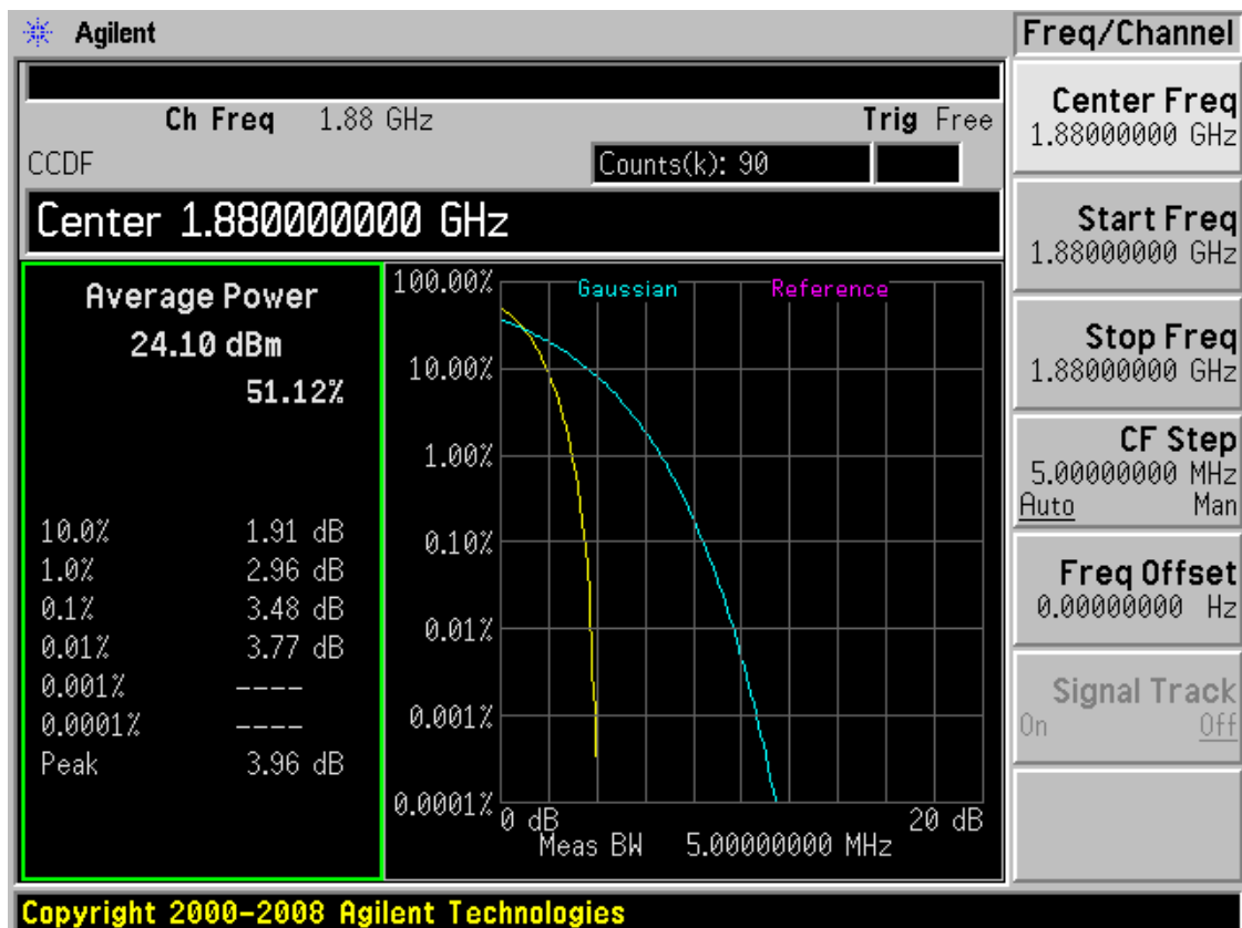
CDMA PCS RC3 (SO32) CH600 Channel
