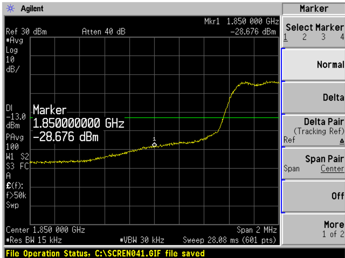
CDMA PCS RC3 (SO32) 25 Channel
