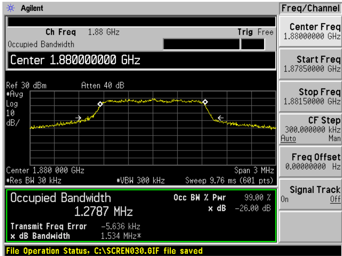
CDMA PCS RC1 (SO2) CH600 Occupied Bandwidth
