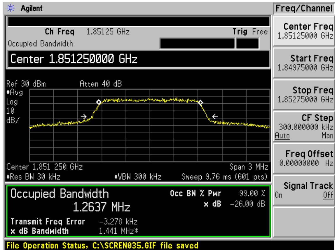
CDMA PCS RC3 (SO32) CH25 Occupied Bandwidth
