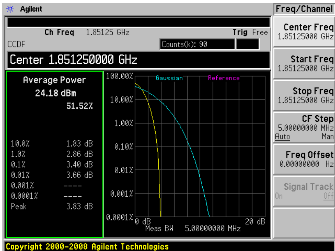
CDMA PCS RC3 (SO32) CH25 Channel
