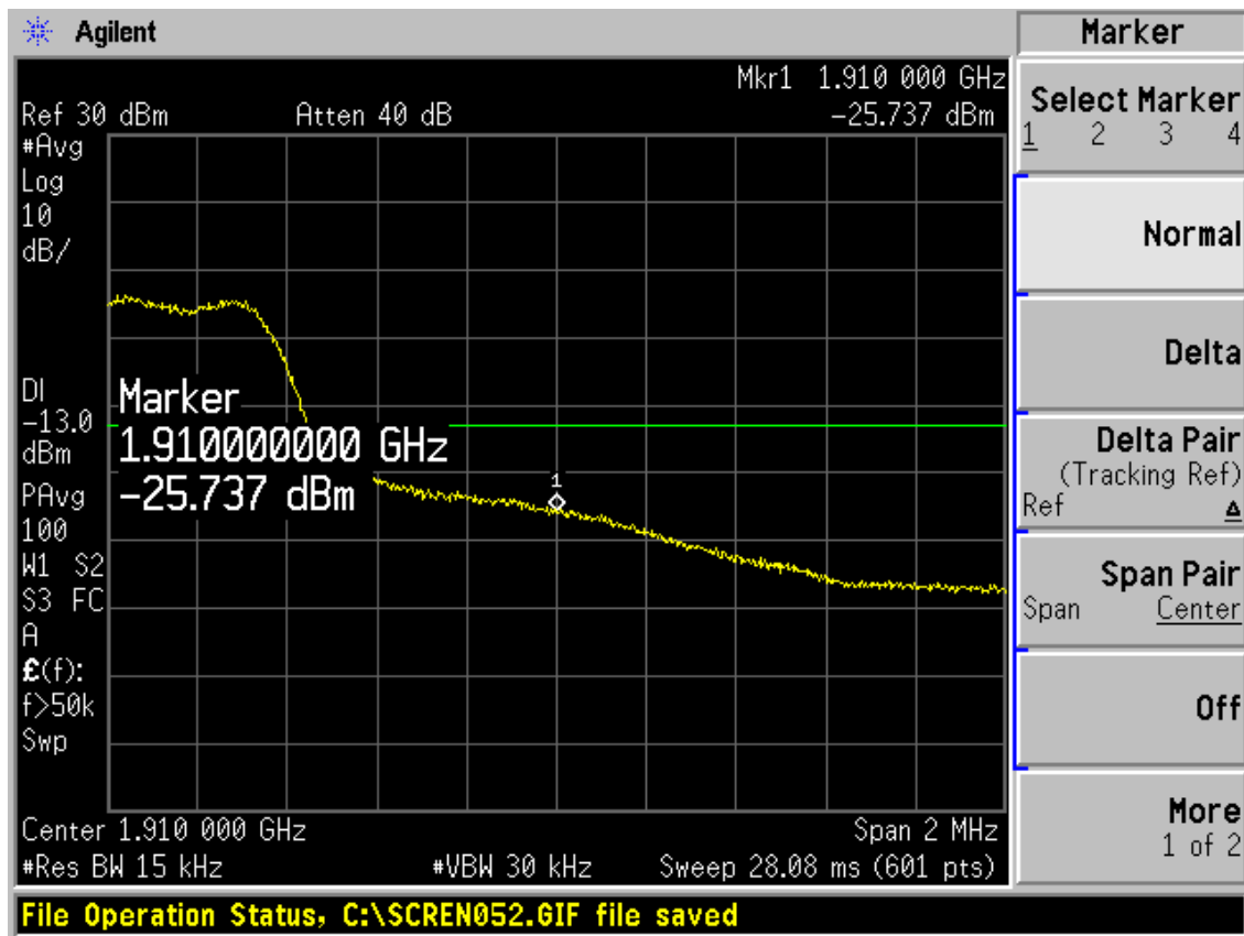
CDMA PCS RC1 (SO2) 1175 Channel
