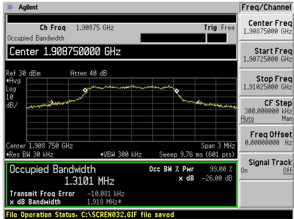
CDMA PCS RC1 (SO2) CH1175 Occupied Bandwidth
