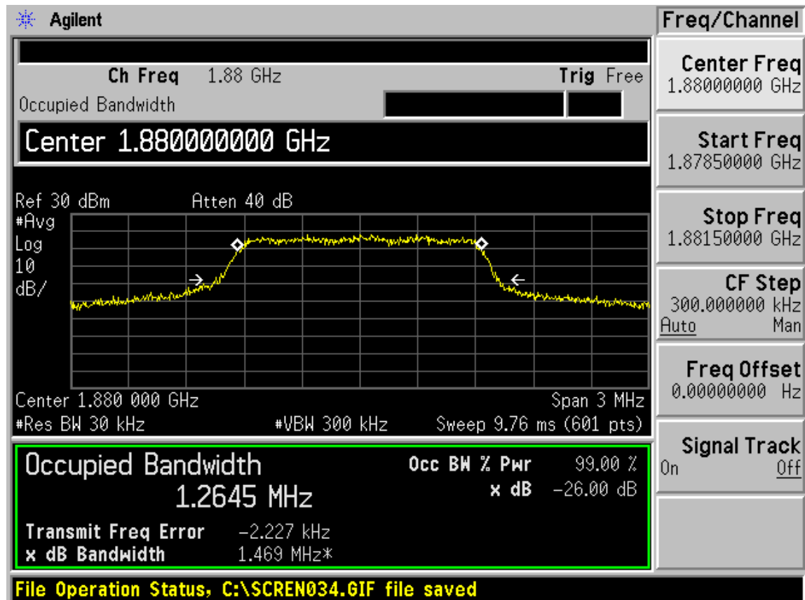
CDMA PCS RC3 (SO32) CH600 Occupied Bandwidth
