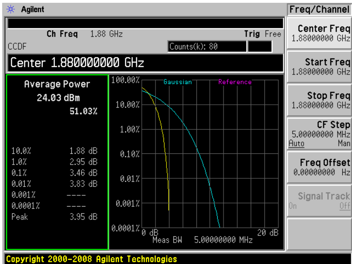
CDMA PCS RC1 (SO2) CH600 Channel
