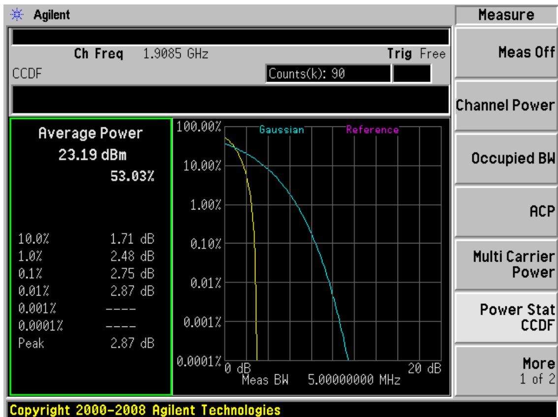
CDMA PCS RC1 (SO2) CH1175 Channel
