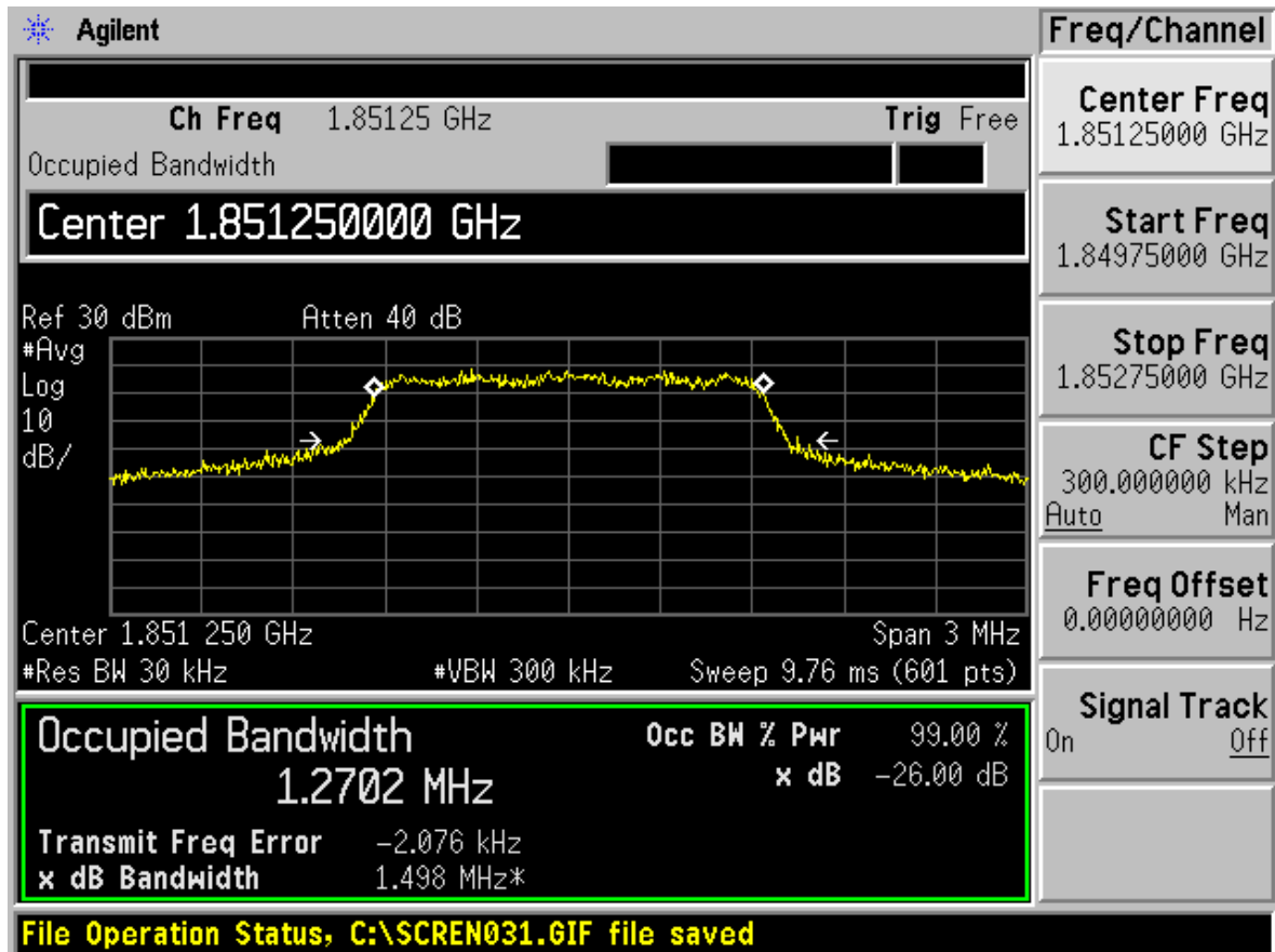
CDMA PCS RC1 (SO2) CH25 Occupied Bandwidth
