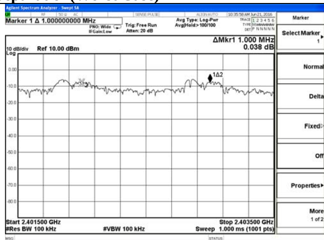
Test Plot of Frequency Separation (2Mbps)
