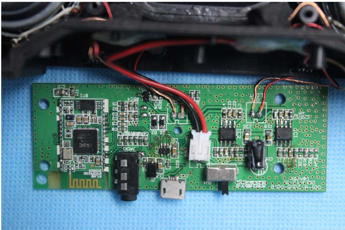
Model: PH-BT1000 Photo 2
