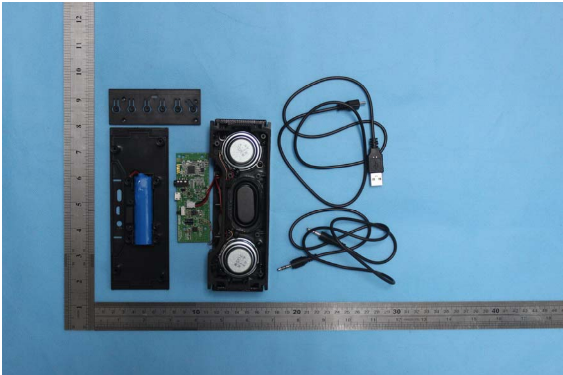
Model: PH-BT1000 Photo 1
