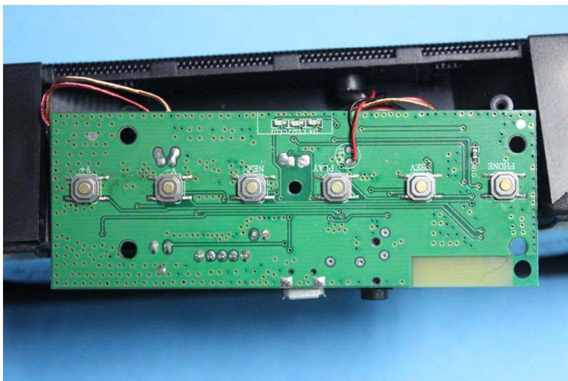
Model: PH-BT1000 Photo 4
