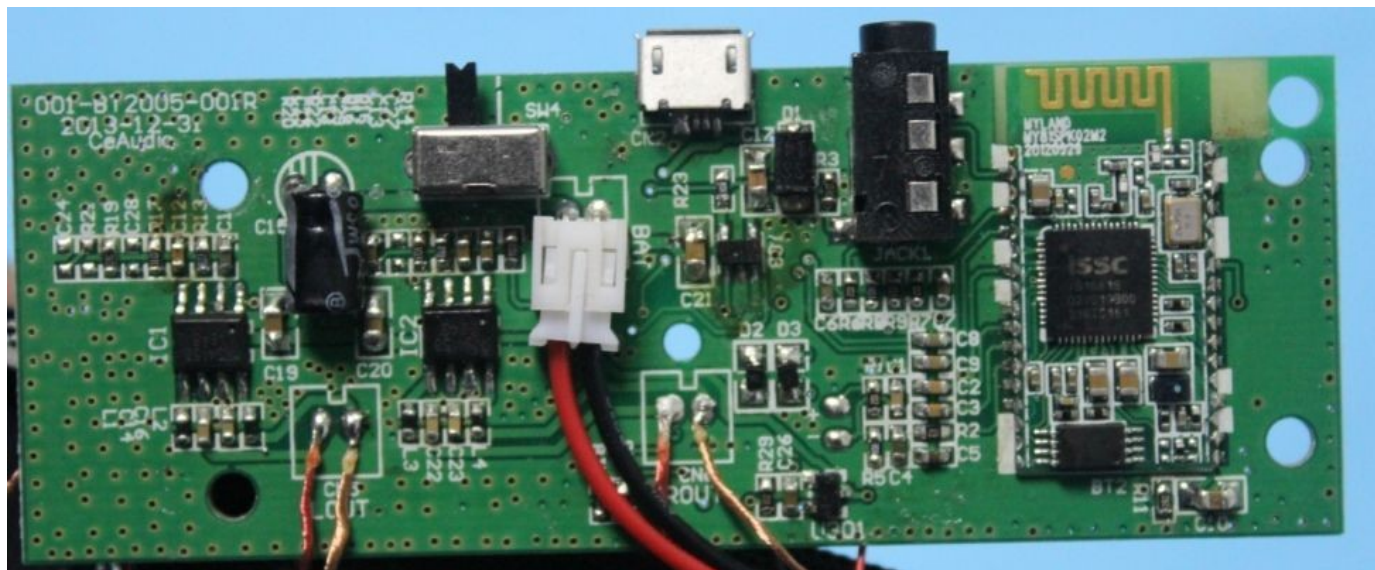
Model: PH-BT1000 Photo 3
