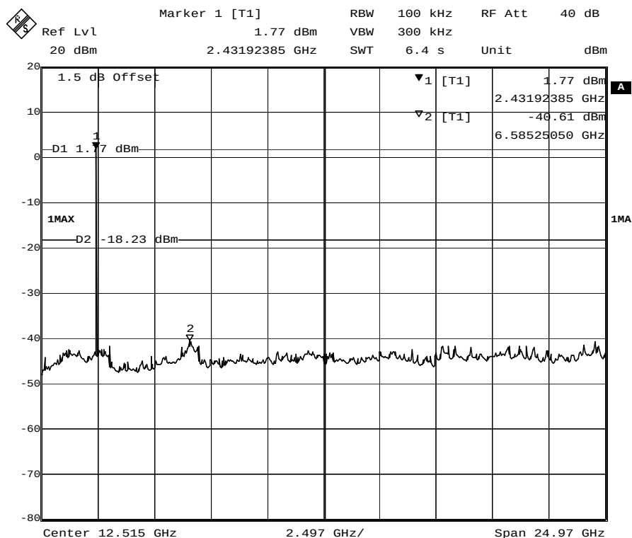
CH39 Data rate 1Mbps
