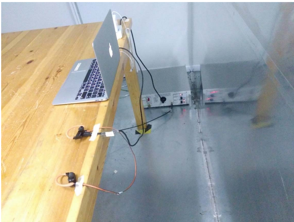
Conducted Emission Test Photo 1
