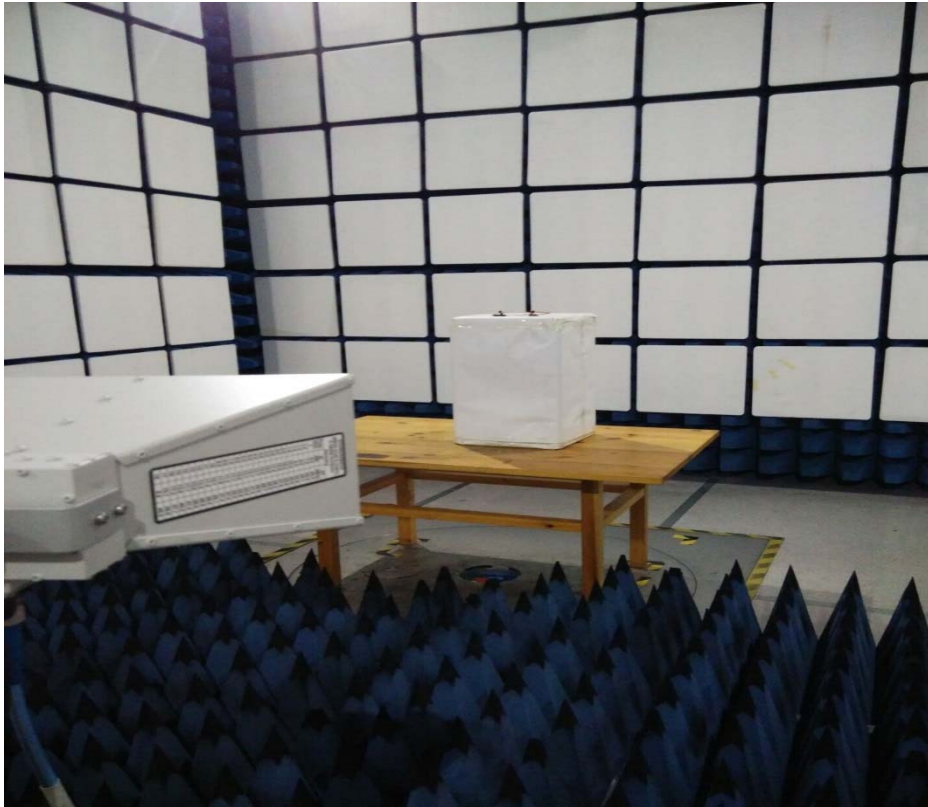
Above 1GHz-1
