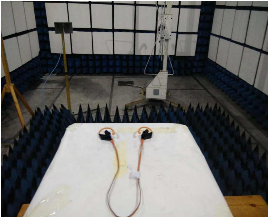
Above 1GHz-1
