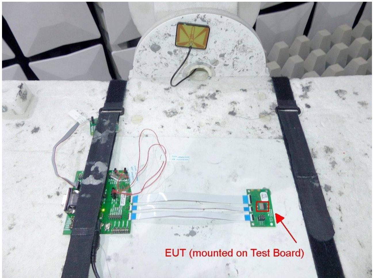
Photo 5: Test setup of EUT and auxiliaries, detail
