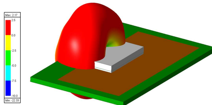
3D radiation pattern @5.5GHz
