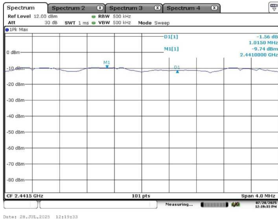
3DH5_2441MHz
