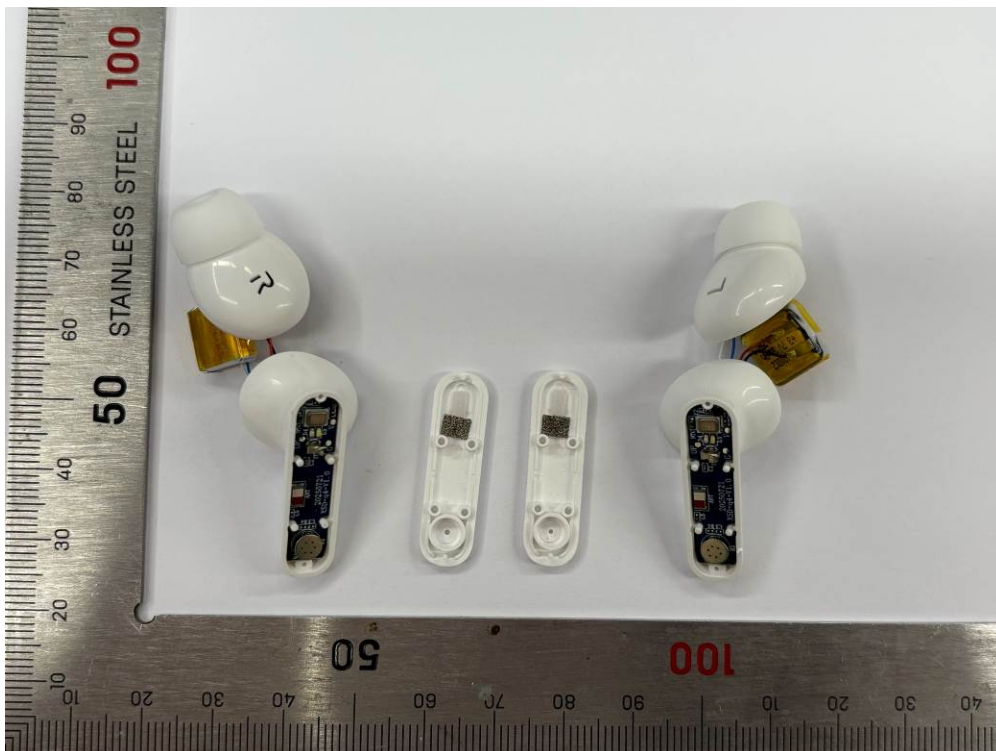
Fig. 4 Internal view of earbuds
