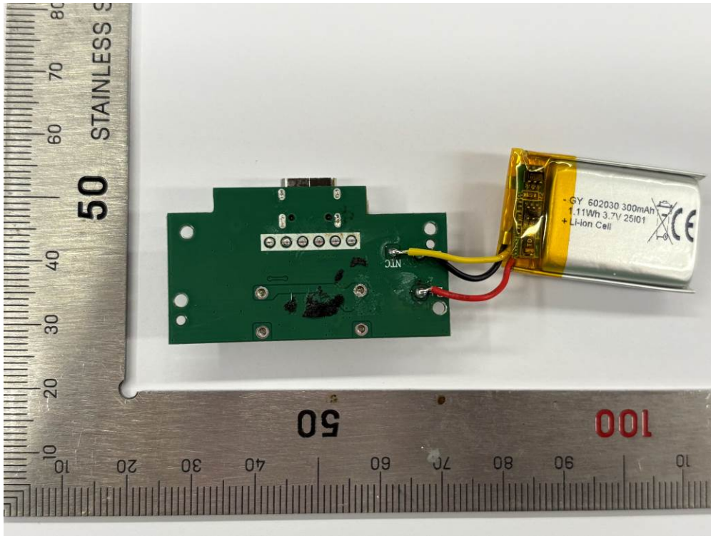
Fig. 3 PCB view of charging case
