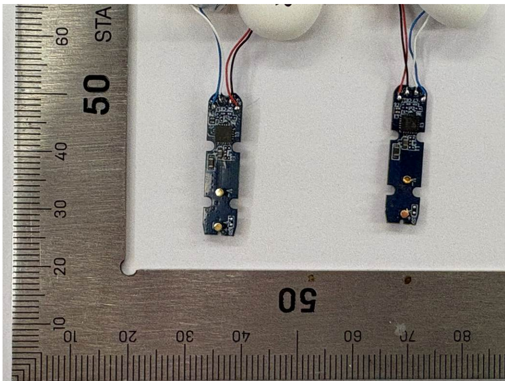
Fig. 6 PCB view of earbuds
