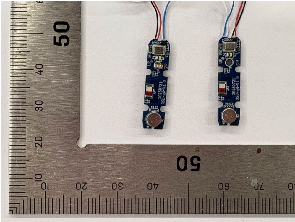
Fig. 5 PCB view of earbuds
