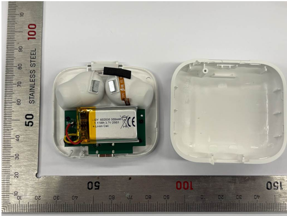
Fig. 1 Internal view of charging case
