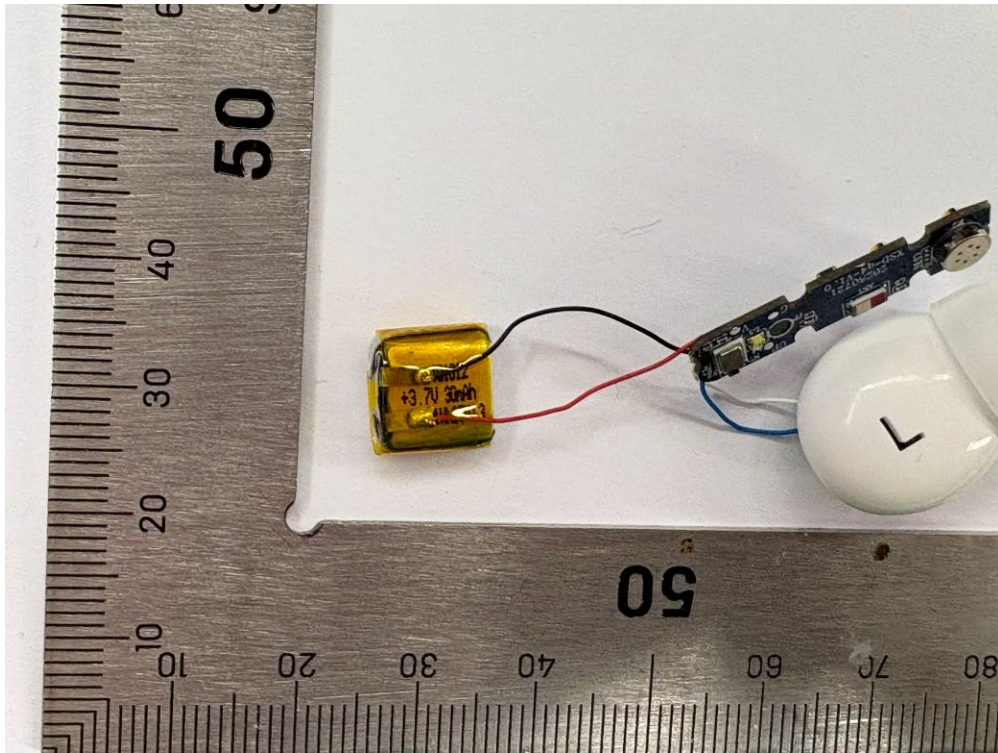
Fig. 7 Battery view of earbuds
