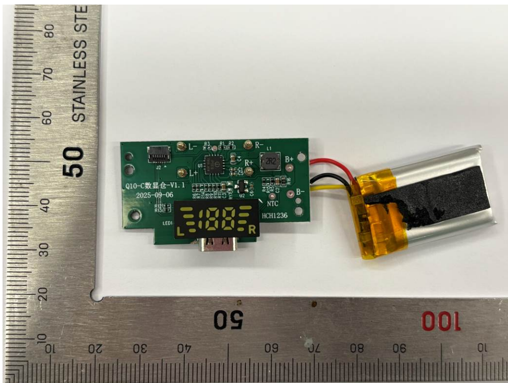
Fig. 2 PCB view of charging case
