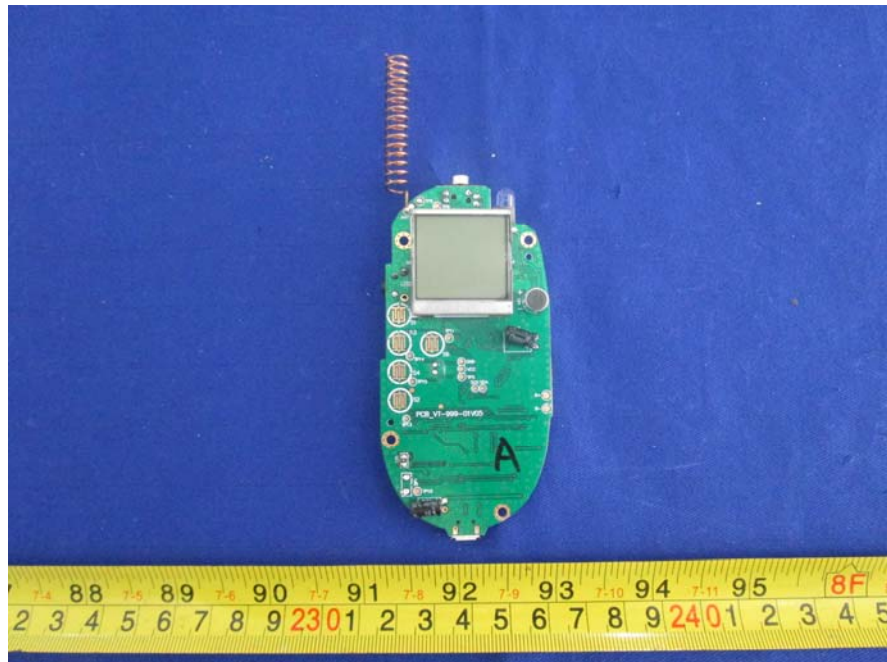
EUT- Circuit Board Top View
