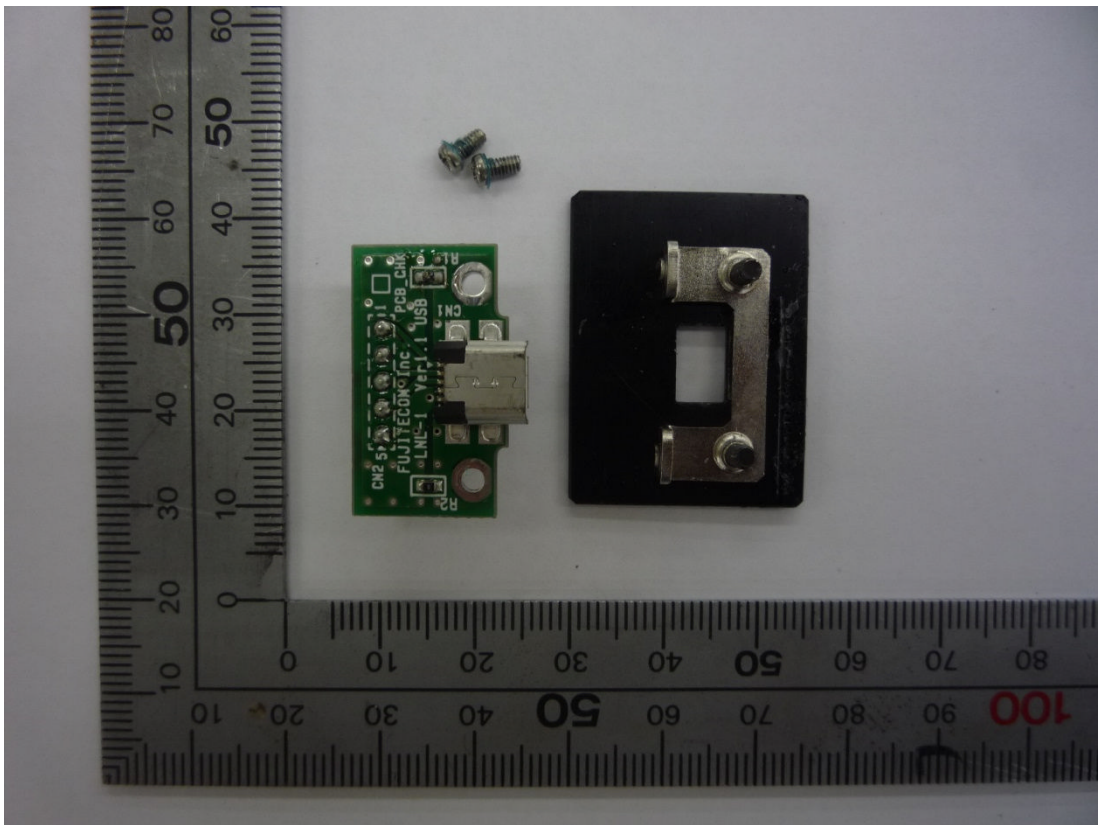
USB assembly
