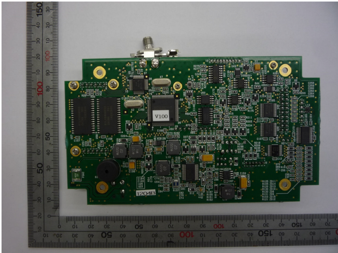
Bottom of main PCB
