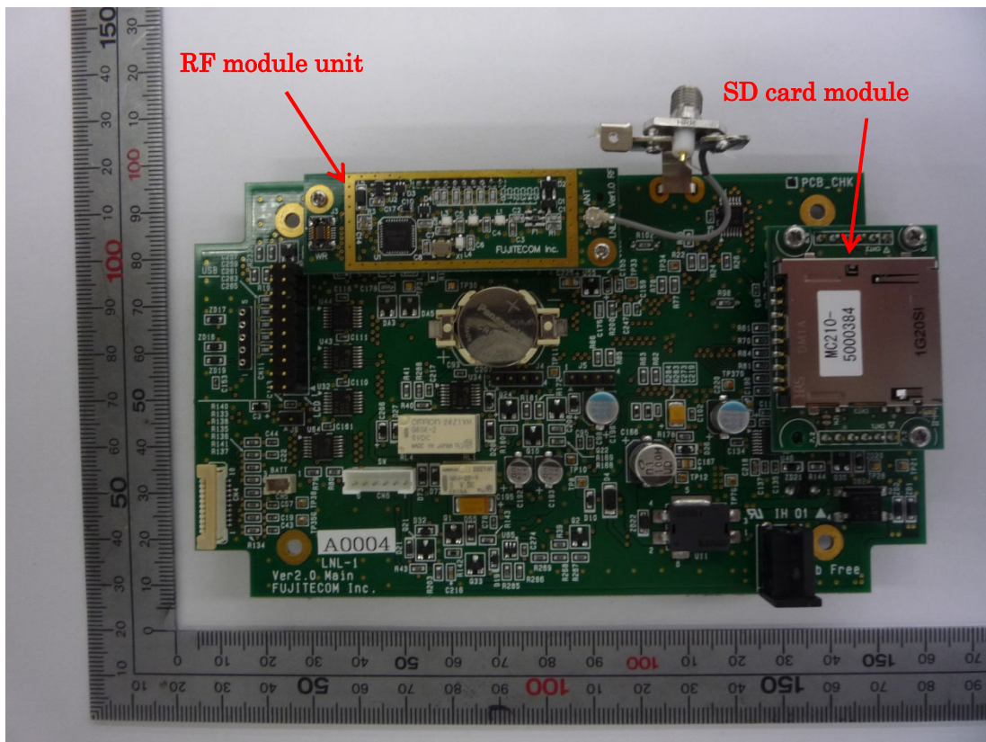
Structure of main PCB
