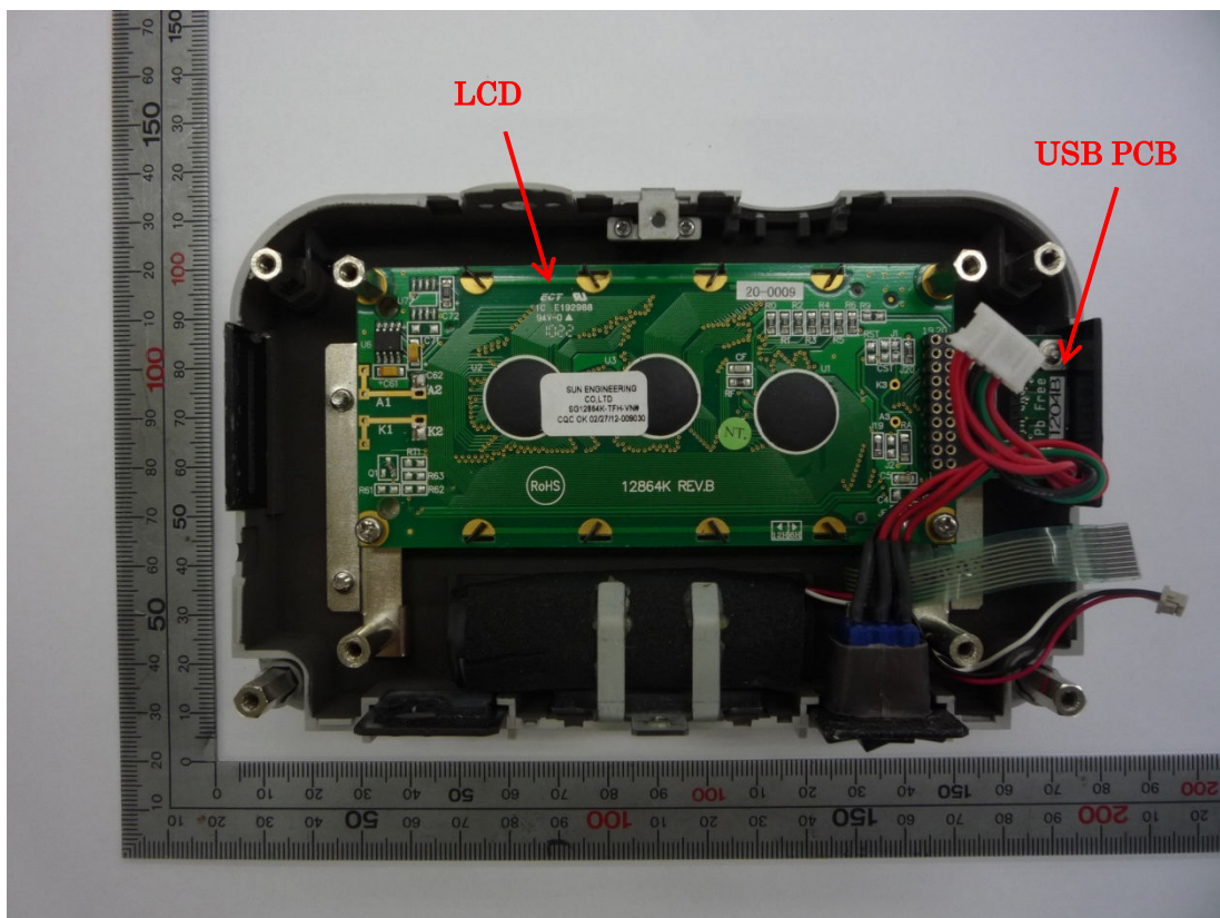
LCD PCB with front case
