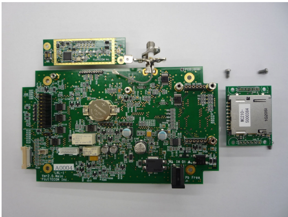
Remove at RF module and SD card module
