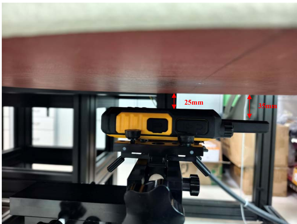
Face Up Setup Photo (25 mm)
