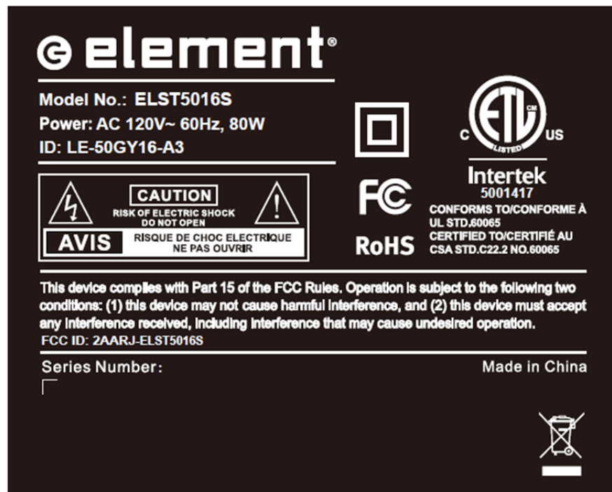
ELST5016S_FCC label and label location
