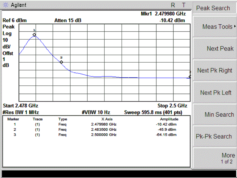
(Plot 4.5.3 A4:Channel 40: 2480MHz)
