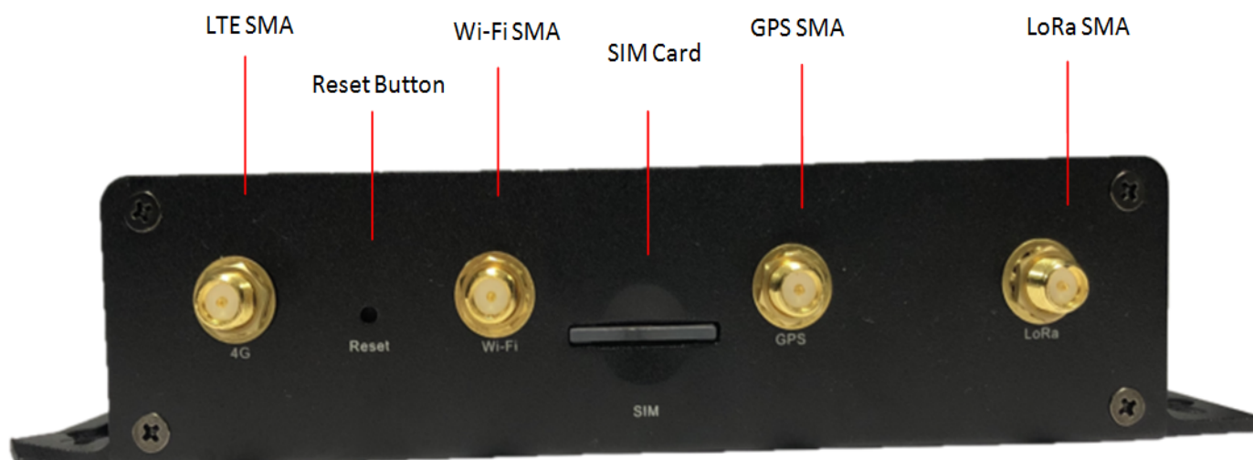
Back Panel -
