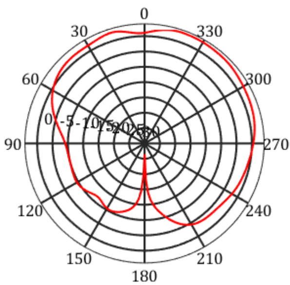
frequency=2500MHz, X-Z Plane
