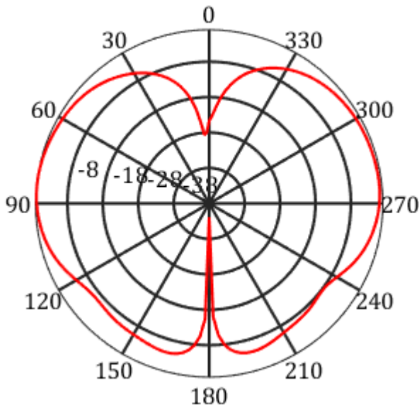
frequency=2500MHz, X-Z Plane
