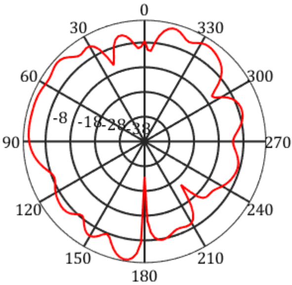
frequency=5150MHz, Y-Z Plane
