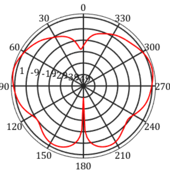
frequency=5150MHz, X-Z Plane
