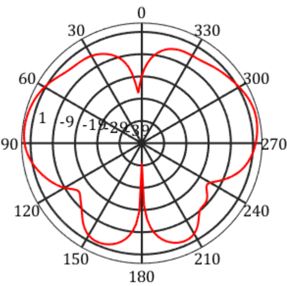
frequency=5850MHz, X-Z Plane
