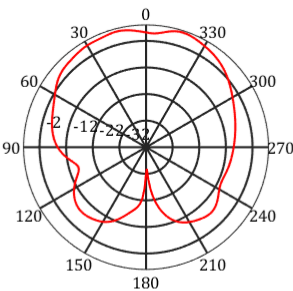
frequency=2450MHz, Y-Z Plane
