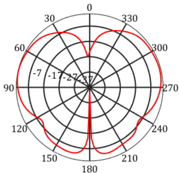
frequency=2400MHz, X-Z Plane
