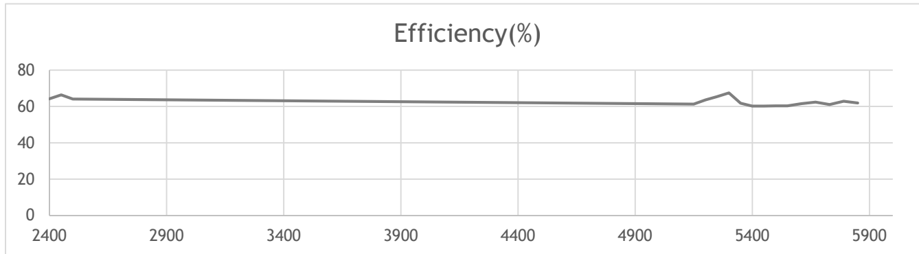
Antenna efficiency
