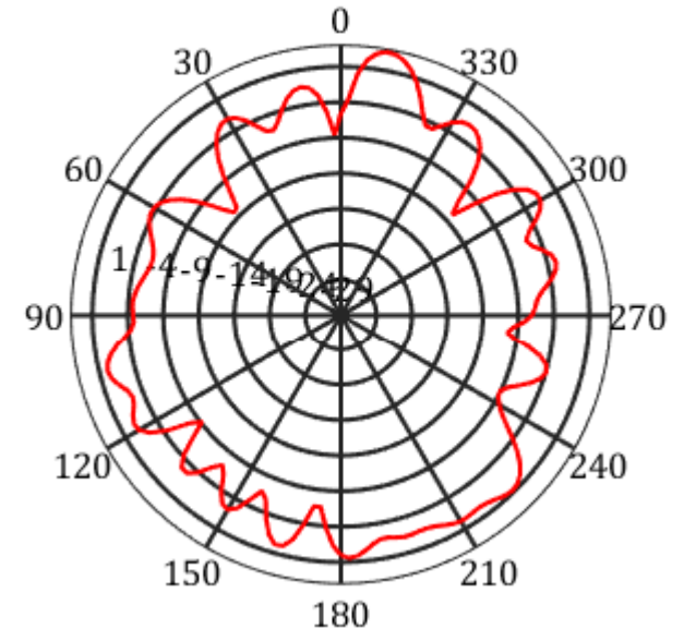
frequency=5850MHz, X-Y Plane
