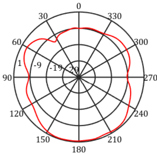
frequency=2500MHz, X-Y Plane
