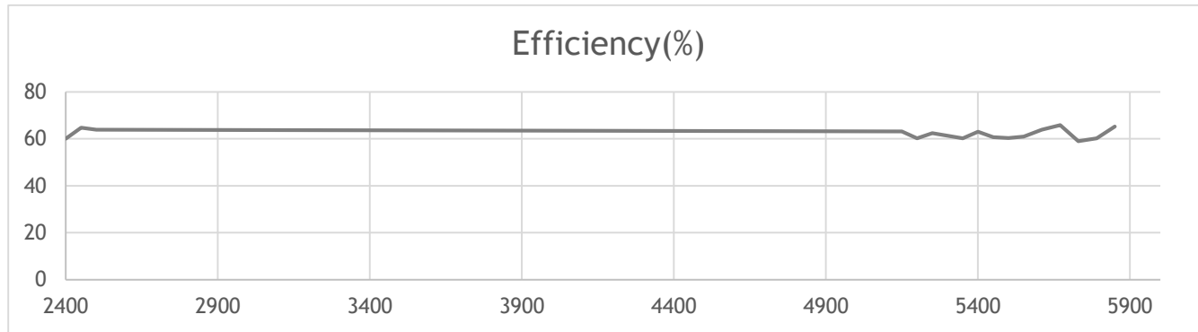
Antenna efficiency
