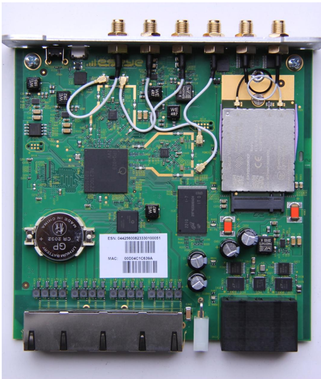
Figure 3: Hera604v6 PCB Top with WiFi Shield Fitted Removed
