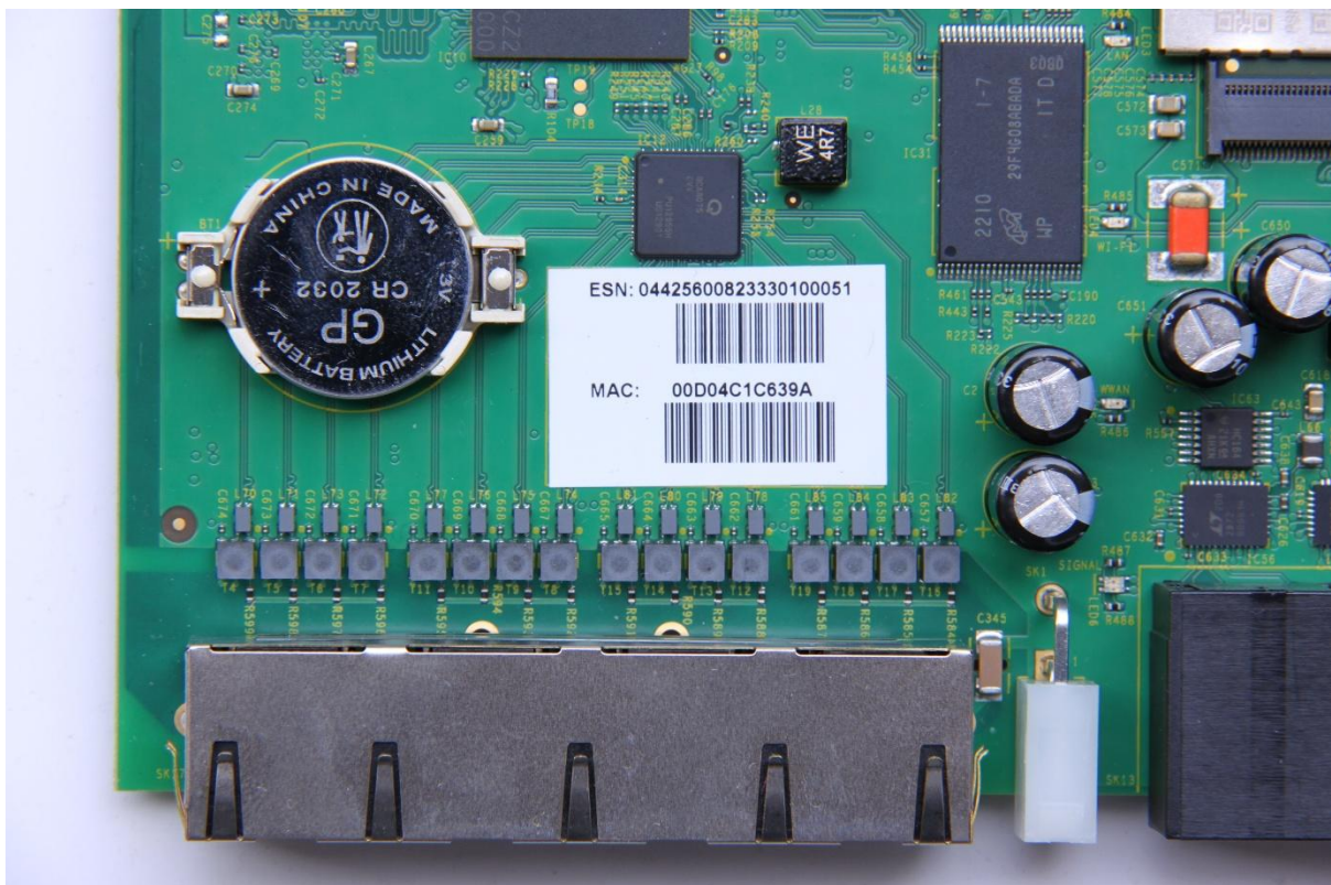
Figure 2a: Hera604v6 PCB Top (close up)
