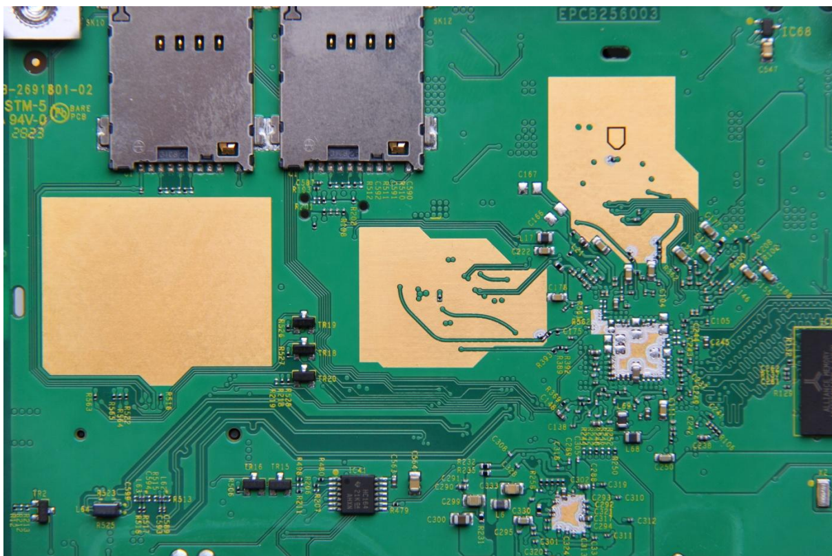
Figure 5a: Hera604v6 PCB Bottom (Thermal Transfer Can removed close up)
