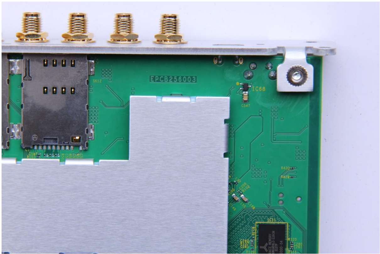
Figure 4d: Hera604v6 PCB Bottom (close up)
