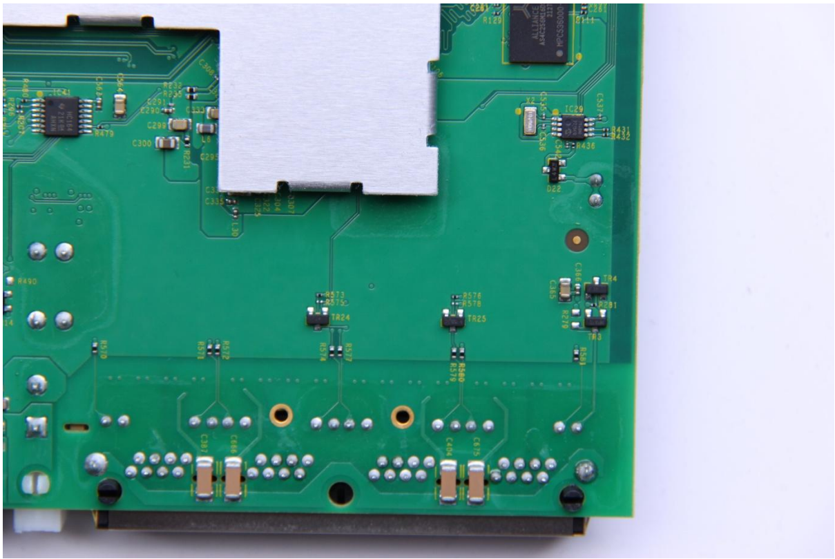
Figure 4b: Hera604v6 PCB Bottom (close up)
