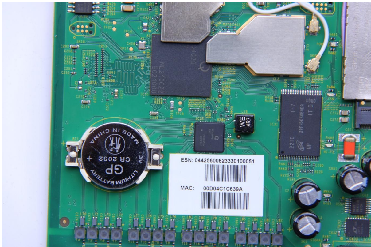
Figure 2g: Hera604v6 PCB Top (close up)
