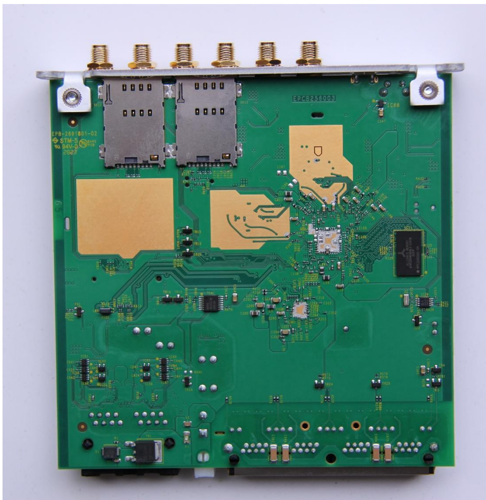
Figure 5: Hera604v6 PCB Bottom (Thermal Transfer Can removed)
