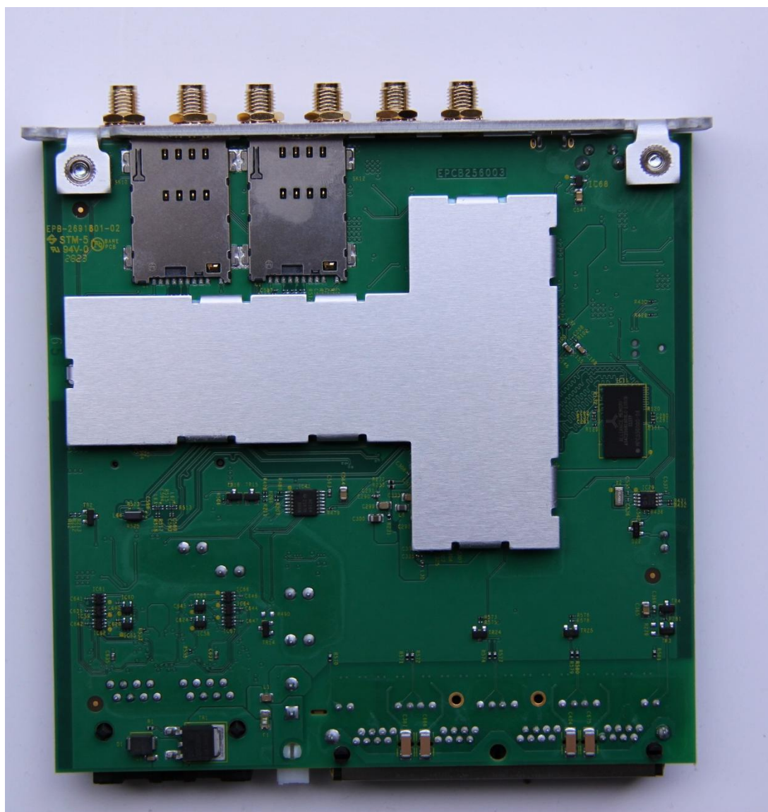
Figure 4: Hera604v6 PCB Bottom
