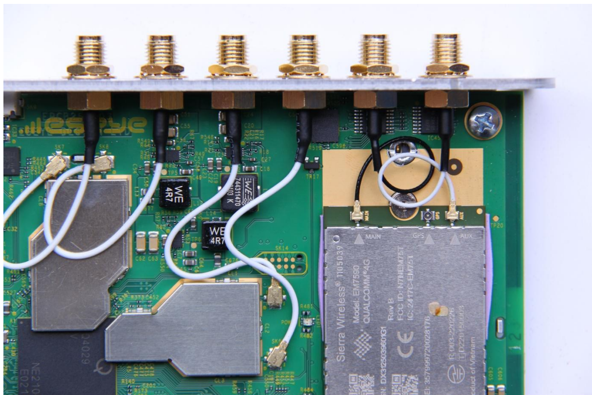
Figure 2e: Hera604v6 PCB Top (close up)
