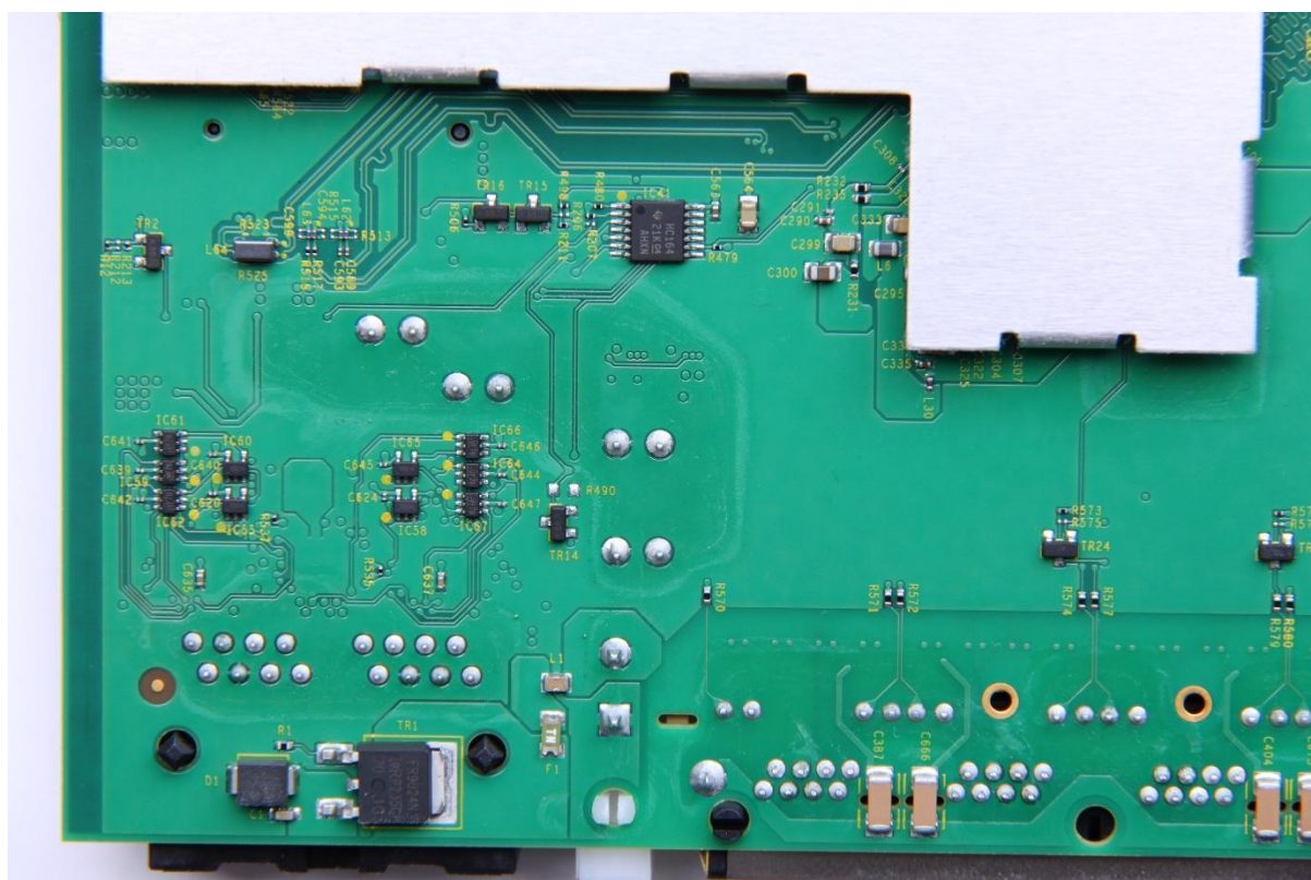
Figure 4a: Hera604v6 PCB Bottom (close up)
