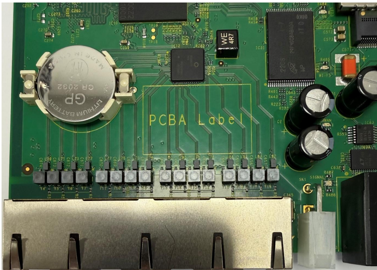
Figure 3b: Hera604v6 PCB Top (close up) – label removed
