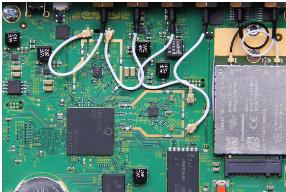
Figure 3a: Hera604v6 PCB Top with WiFi Shield Fitted Removed (close up)
