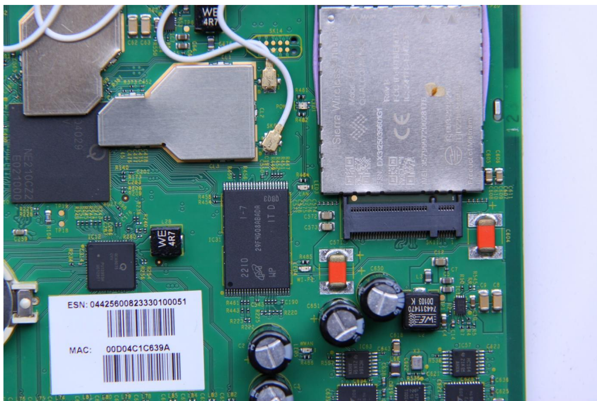
Figure 2d: Hera604v6 PCB Top (close up)
