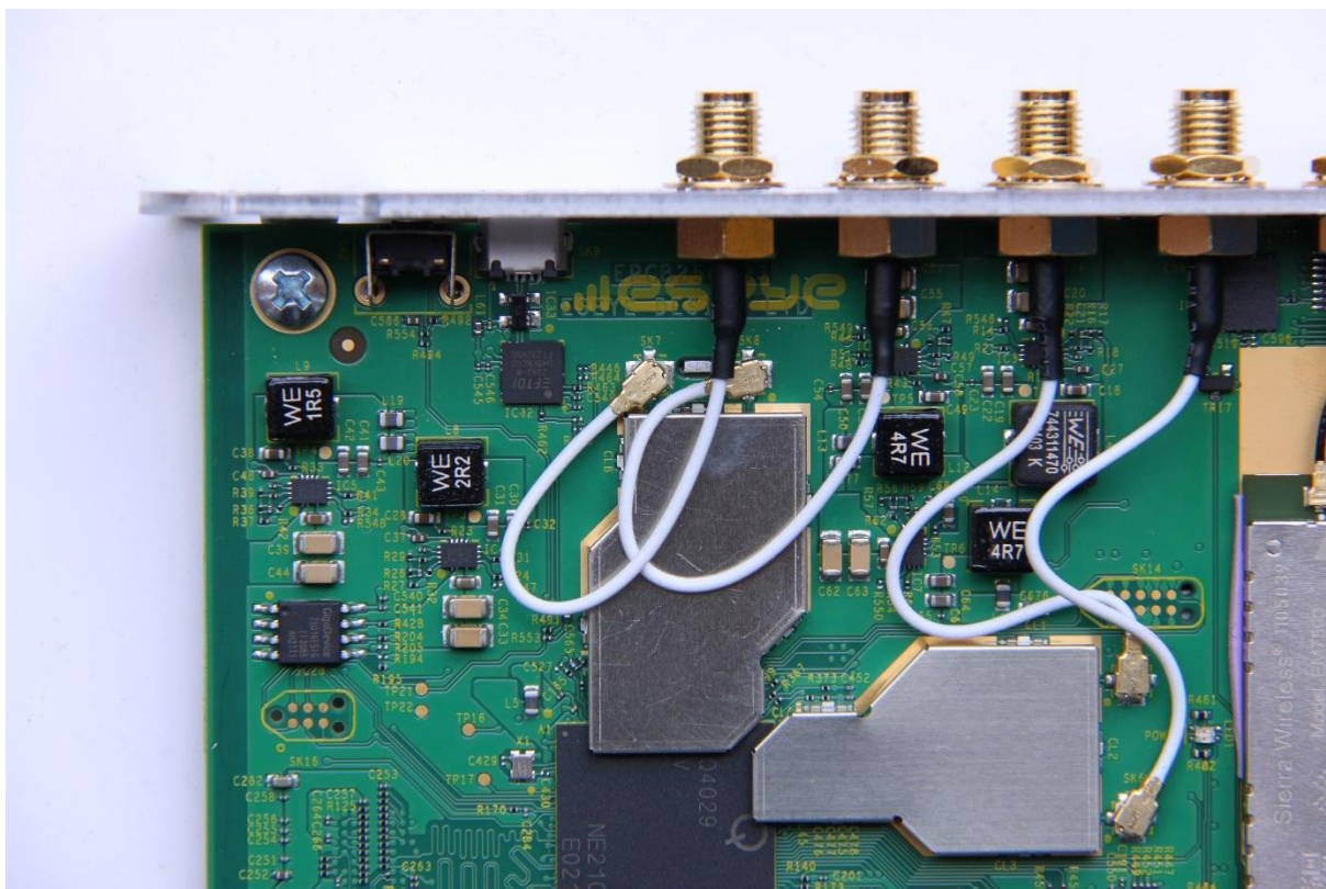
Figure 2f: Hera604v6 PCB Top (close up)
