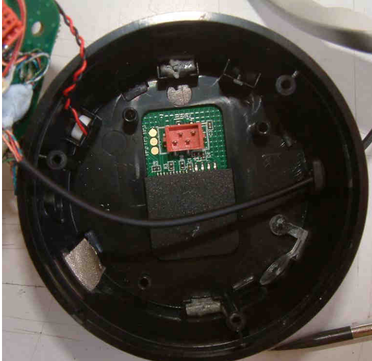
Internal view of cup (Speaker 2 removed, main PCB removed)
