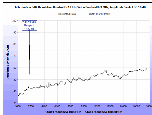
Plot 24. Radiated Spurious Emissions, 1GHz - 18 GHz, High Channel Peak
