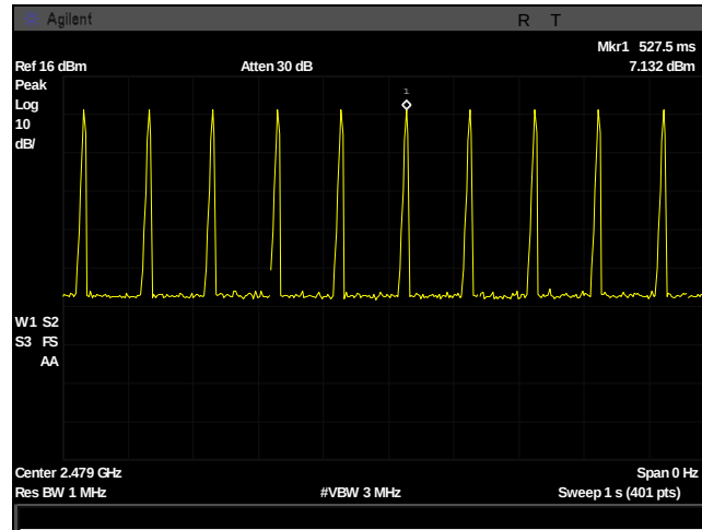
Plot 4. Dwell Time - Number of Hops in 1 Second
