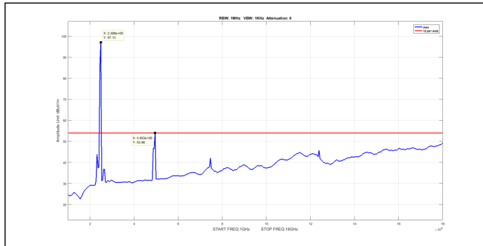
Plot 35. Simultaneous Average Spurious Emission 1-18GHz, BW 40M, Ch 2437M, B mode, BT high Channel
