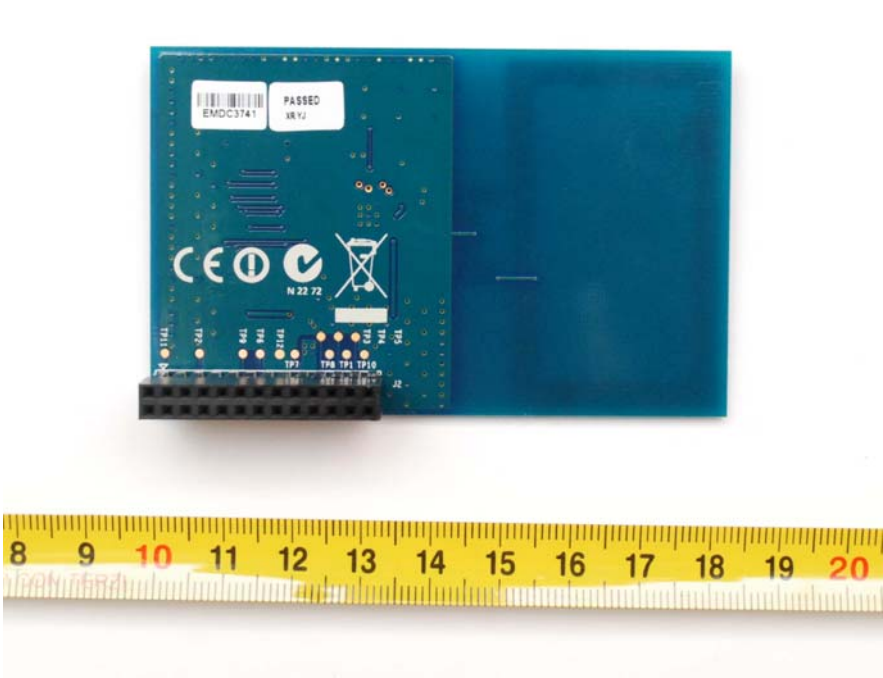
Picture 2: EXPLORE-NFC board - bottom side
