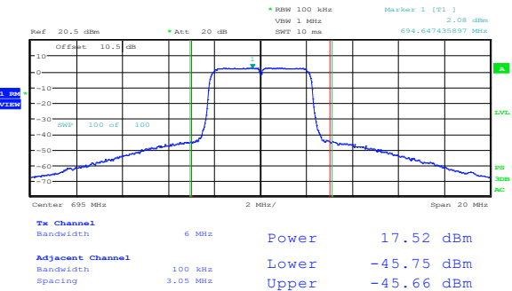
Figure 8.4-6: Adjacent channel power on high channel, 64-QAM
