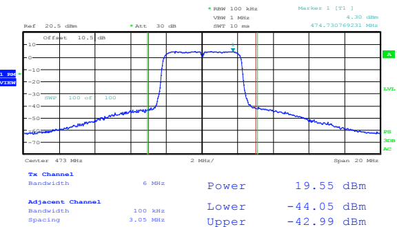
Figure 8.2-2: Output power on low channel, 64-QAM
