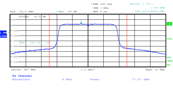
Figure 8.2-4: Output power on mid channel, 64-QAM
