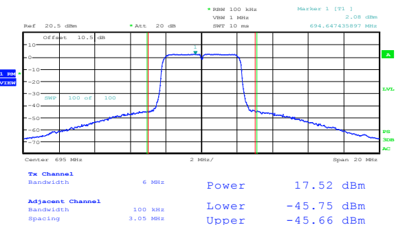
Figure 8.2-6: Output power on high channel, 64-QAM
