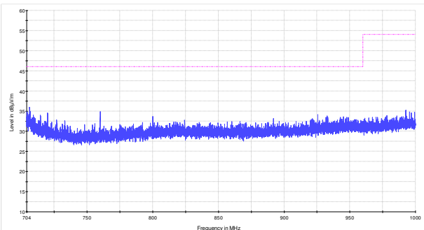
Figure 8.6-4: Radiated spurious emissions within 704–1000 MHz for upper channel for Omnidirectional antenna
