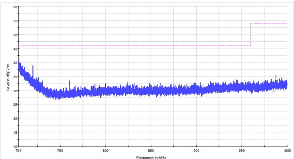
Figure 8.6-8: Radiated spurious emissions within 704–1000 MHz for upper channel for Directional antenna
