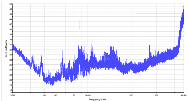
Figure 8.6-5: Radiated spurious emissions within 30–464 MHz for low channel for Directional antenna
