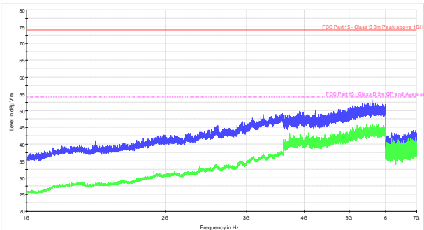
Figure 8.6-10: Radiated spurious emissions within 1–7 GHz for high channel for Omnidirectional antenna
