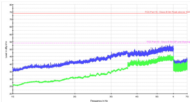
Figure 8.6-9: Radiated spurious emissions within 1–7 GHz for low channel for Omnidirectional antenna
