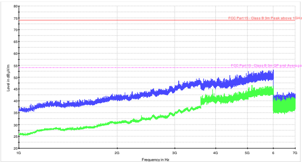
Figure 8.6-12: Radiated spurious emissions within 1–7 GHz for high channel for Directional antenna
