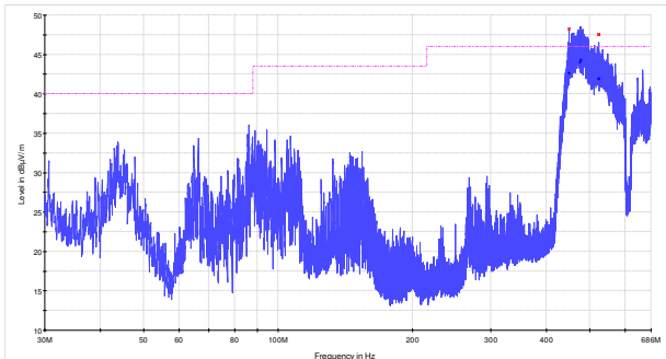
Figure 8.6-7: Radiated spurious emissions within 30–686 MHz for upper channel for Directional antenna
