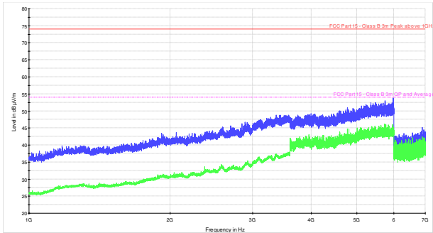
Figure 8.6-11: Radiated spurious emissions within 1–7 GHz for low channel for Directional antenna
