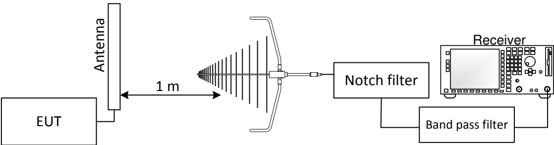
Figure 8.7-1: Setup diagram for 602–620 MHz radiated emissions measurements
