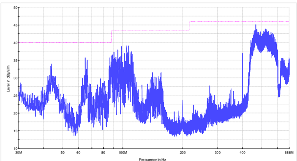
Figure 8.6-3: Radiated spurious emissions within 30–686 MHz for upper channel for Omnidirectional antenna
