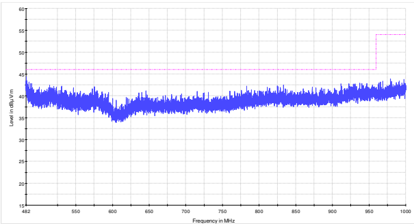
Figure 8.6-2: Radiated spurious emissions within 482–1000 MHz for low channel for Omnidirectional antenna
