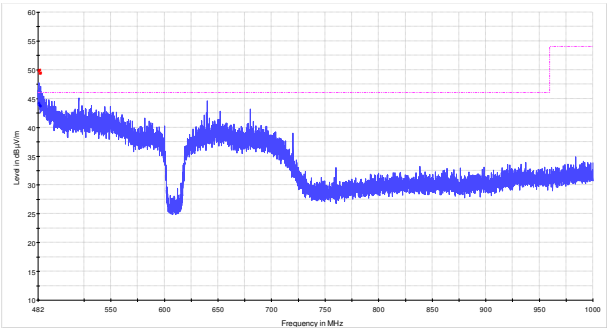
Figure 8.6-6: Radiated spurious emissions within 482–1000 MHz for low channel for Directional antenna
