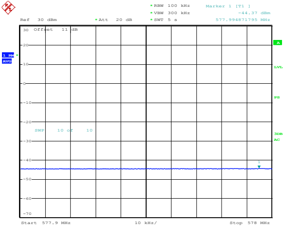
Figure 8.5-1: Lower band edge for low channel
