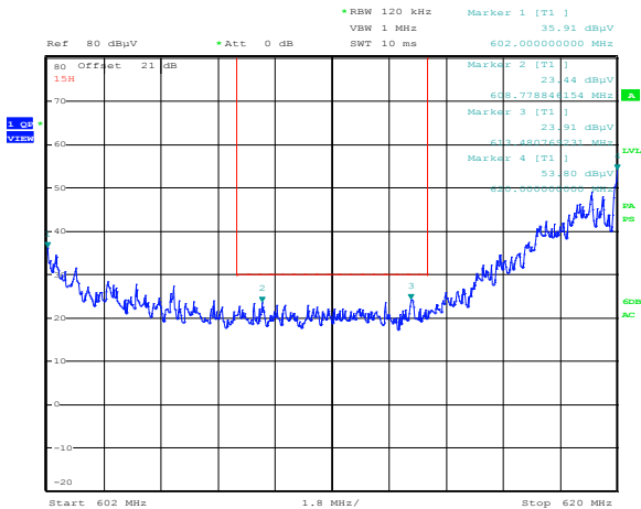
Figure 8.7-3: Radiated spurious emissions within 602–620 MHz for upper adjacent channel to the restricted band (623 MHz), Omnidirectional antenna
