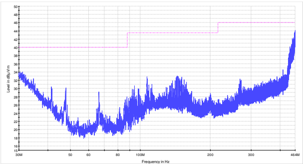
Figure 8.6-1: Radiated spurious emissions within 30–464 MHz for low channel for Omnidirectional antenna
