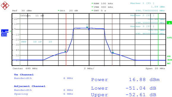
Figure 8.4-3: Adjacent channel power for high channel
