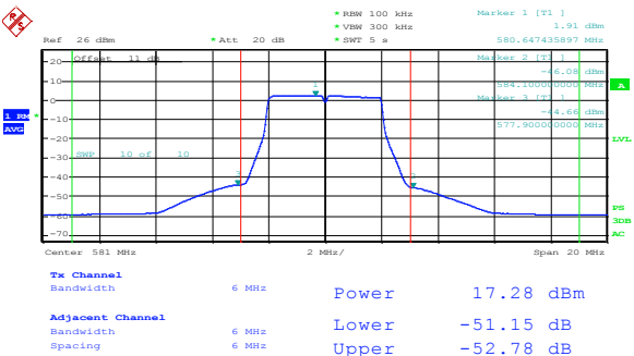
Figure 8.4-2: Adjacent channel power for mid channel
