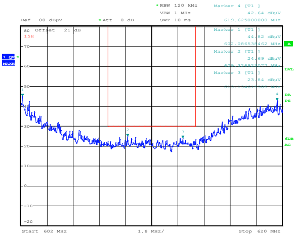
Figure 8.7-2: Radiated spurious emissions within 602–620 MHz for lower adjacent channel to the restricted band (599 MHz), Omnidirectional antenna
