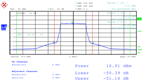
Figure 8.4-1: Adjacent channel power for low channel
