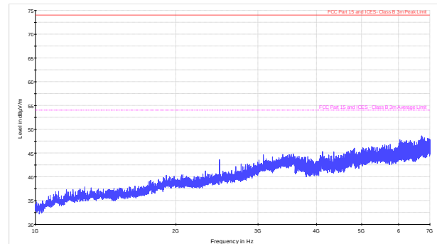
Figure 8.9-34: Radiated spurious emissions within 1–7 GHz for low channel for Panel antenna (BTS)
