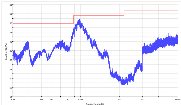
Figure 8.9-9: Radiated spurious emissions within 30–566 MHz for mid channel for Panel antenna (BTS)
