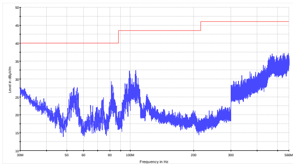
Figure 8.9-27: Radiated spurious emissions within 30–566 MHz for mid channel for Omnidirectional antenna (CPE)
