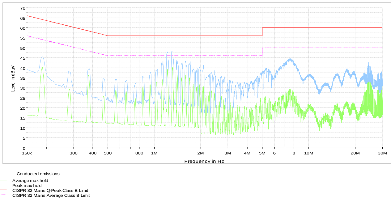
Plot 8.4-2: Conducted emissions on neutral line (BTS)
