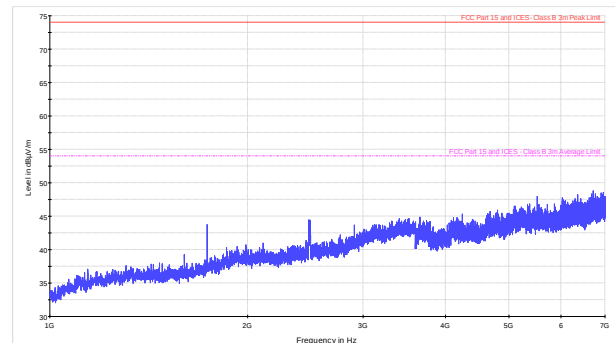
Figure 8.9-36: Radiated spurious emissions within 1–7 GHz for high channel for Panel antenna (BTS)
