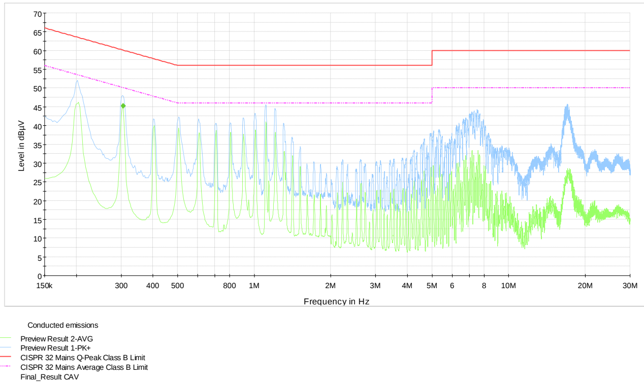
Plot 8.4-4: Conducted emissions on neutral line (CPE)
