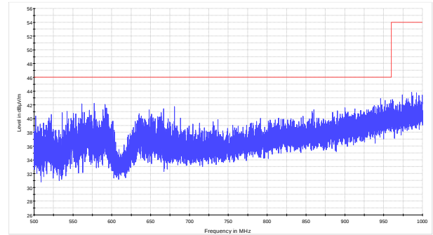
Figure 8.9-20: Radiated spurious emissions within 500–1000 MHz for low channel for Panel antenna (CPE)
