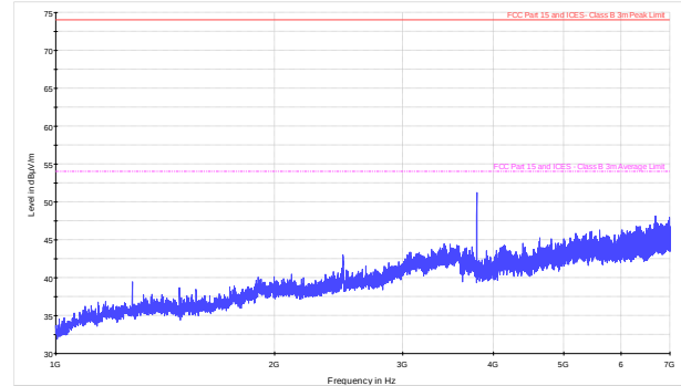
Figure 8.9-44: Radiated spurious emissions within 1–7 GHz for mid channel for Omnidirectional antenna (CPE)
