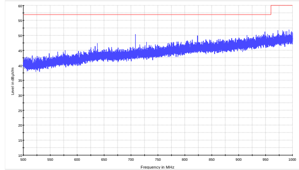
Figure 8.9-8: Radiated spurious emissions within 500–1000 MHz for low channel for Panel antenna (BTS)
