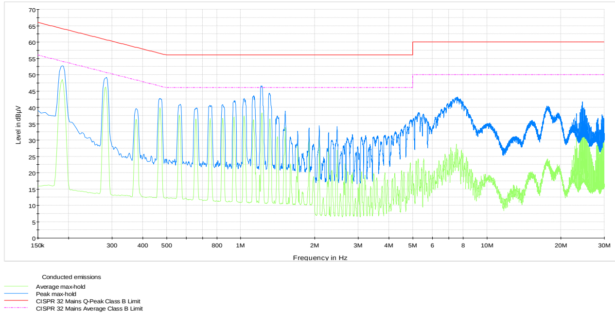
Plot 8.4-1: Conducted emissions on phase line (BTS)
