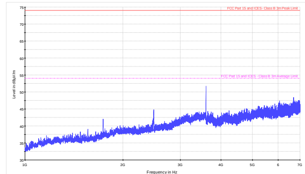
Figure 8.9-42: Radiated spurious emissions within 1–7 GHz for high channel for Panel antenna (CPE)
