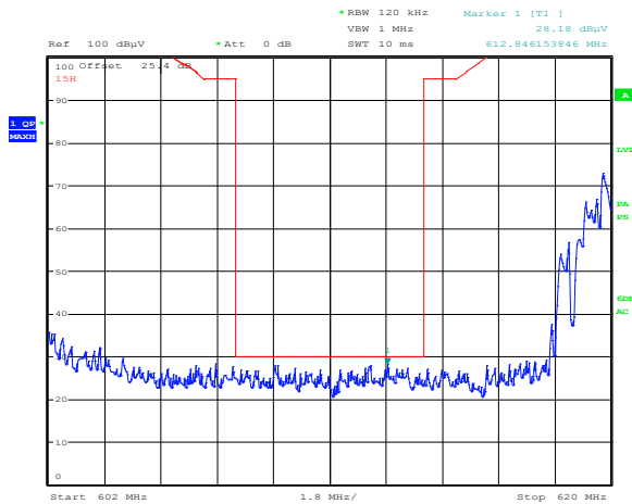
Figure 8.10-3: Radiated spurious emissions within 602–620 MHz for upper adjacent channel to the restricted band, LPDA antenna
