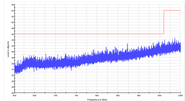
Figure 8.9-28: Radiated spurious emissions within 602–1000 MHz for mid channel for Omnidirectional antenna (B CPE TS)
