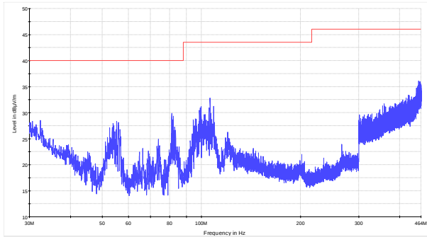
Figure 8.9-25: Radiated spurious emissions within 30–464 MHz for low channel for Omnidirectional antenna (CPE)
