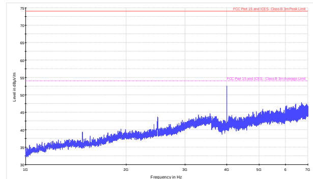
Figure 8.9-40: Radiated spurious emissions within 1–7 GHz for low channel for Panel antenna (CPE)
