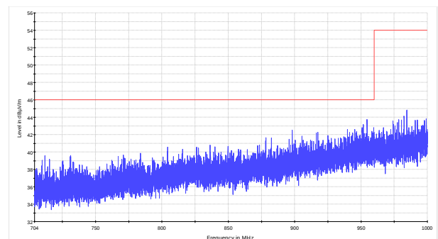
Figure 8.9-24: Radiated spurious emissions within 704–1000 MHz for high channel for Panel antenna (CPE)
