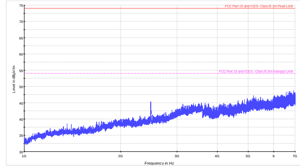
Figure 8.9-32: Radiated spurious emissions within 1–7 GHz for mid channel for LPDA antenna (BTS)
