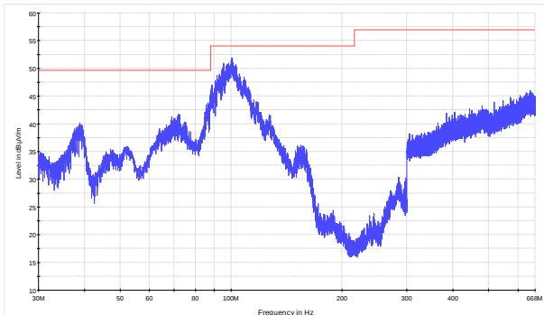
Figure 8.9-11: Radiated spurious emissions within 30–668 MHz for high channel for Panel antenna (BTS)
