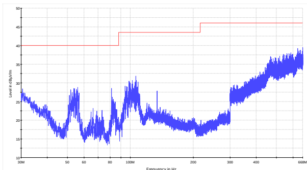
Figure 8.9-29: Radiated spurious emissions within 30–668 MHz for high channel for Omnidirectional antenna (CPE)
