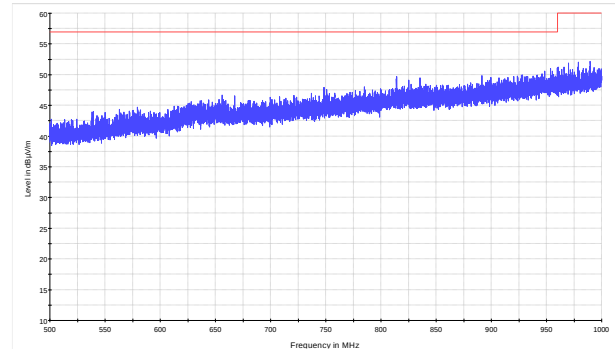
Figure 8.9-2: Radiated spurious emissions within 500–1000 MHz for low channel for LPDA antenna (BTS)
