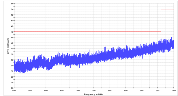
Figure 8.9-26: Radiated spurious emissions within 500–1000 MHz for low channel for Omnidirectional antenna (CPE)
