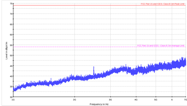
Figure 8.9-31: Radiated spurious emissions within 1–7 GHz for low channel for LPDA antenna (BTS)
