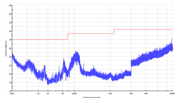
Figure 8.9-17: Radiated spurious emissions within 30–668 MHz for high channel for LPDA antenna (CPE)
