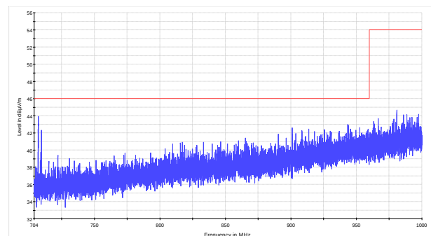
Figure 8.9-18: Radiated spurious emissions within 704–1000 MHz for high channel for LPDA antenna (CPE)
