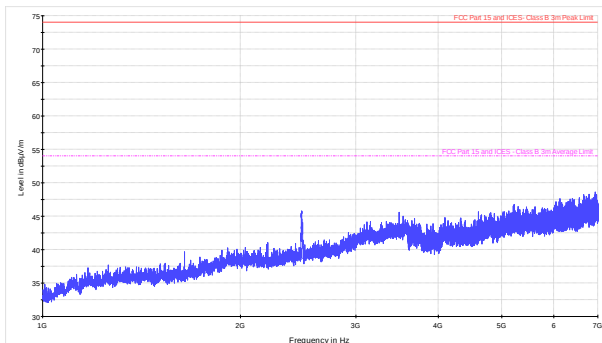
Figure 8.9-35: Radiated spurious emissions within 1–7 GHz for mid channel for Panel antenna (BTS)
