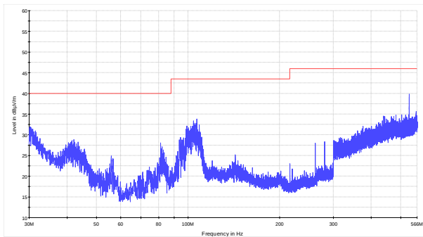
Figure 8.9-15: Radiated spurious emissions within 30–566 MHz for mid channel for LPDA antenna (CPE)
