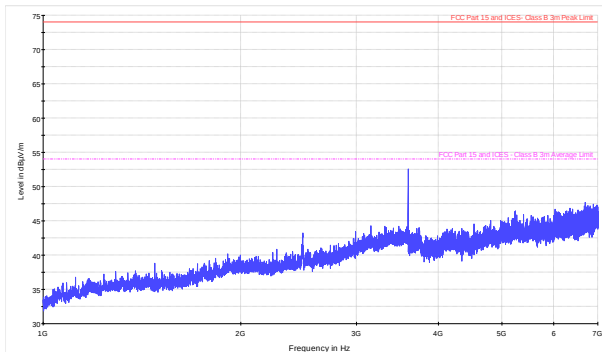
Figure 8.9-39: Radiated spurious emissions within 1–7 GHz for high channel for LPDA antenna (CPE)
