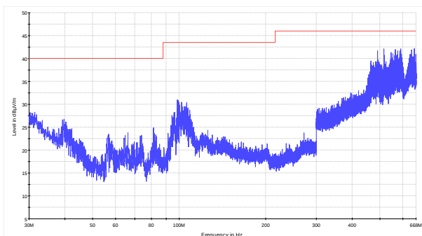
Figure 8.9-23: Radiated spurious emissions within 30–668 MHz for high channel for Panel antenna (CPE)
