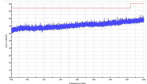
Figure 8.9-10: Radiated spurious emissions within 602–1000 MHz for mid channel for Panel antenna (BTS)
