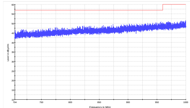
Figure 8.9-12: Radiated spurious emissions within 704–1000 MHz for high channel for Panel antenna (BTS)
