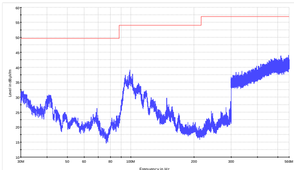
Figure 8.9-3: Radiated spurious emissions within 30–566 MHz for mid channel for LPDA antenna (BTS)
