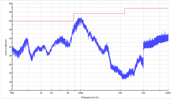
Figure 8.9-7: Radiated spurious emissions within 30–464 MHz for low channel for Panel antenna (BTS)
