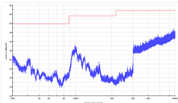
Figure 8.9-5: Radiated spurious emissions within 30–668 MHz for high channel for LPDA antenna (BTS)
