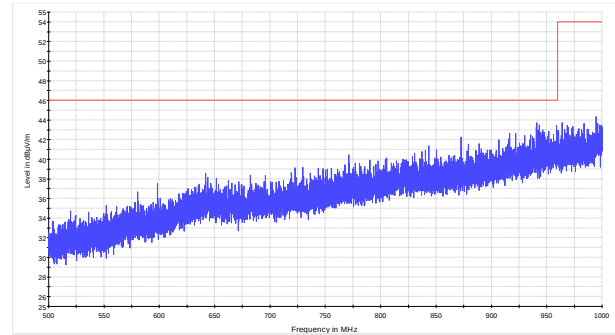
Figure 8.9-14: Radiated spurious emissions within 500–1000 MHz for low channel for LPDA antenna (CPE)
