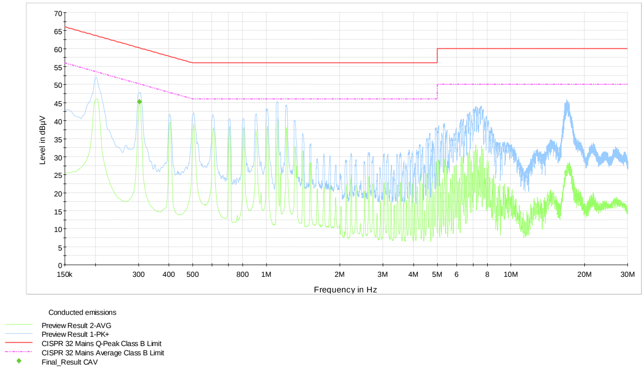
Plot 8.4-3: Conducted emissions on phase line (CPE)
