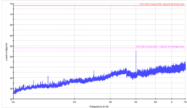
Figure 8.9-43: Radiated spurious emissions within 1–7 GHz for low channel for Omnidirectional antenna (CPE)
