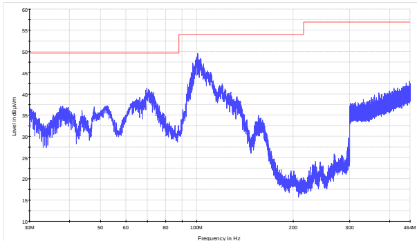
Figure 8.9-1: Radiated spurious emissions within 30–464 MHz for low channel for LPDA antenna (BTS)
