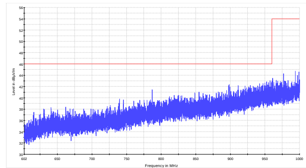
Figure 8.9-16: Radiated spurious emissions within 602–1000 MHz for mid channel for LPDA antenna (CPE)
