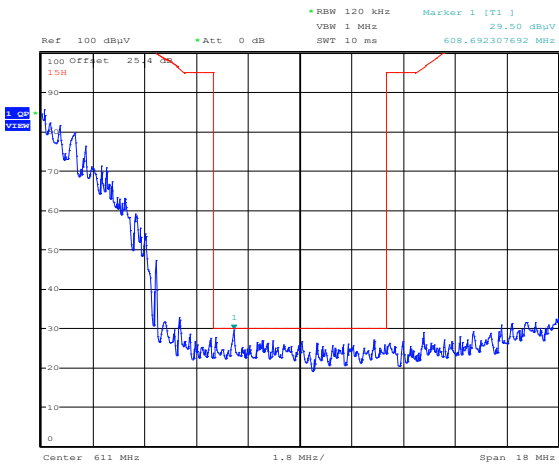
Figure 8.10-2: Radiated spurious emissions within 602–620 MHz for lower adjacent channel to the restricted band, LPDA antenna
