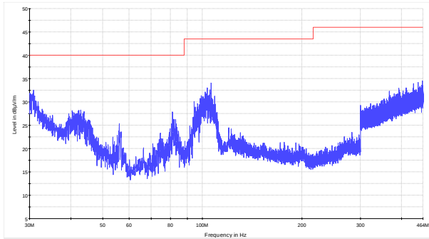
Figure 8.9-13: Radiated spurious emissions within 30–464 MHz for low channel for LPDA antenna (CPE)
