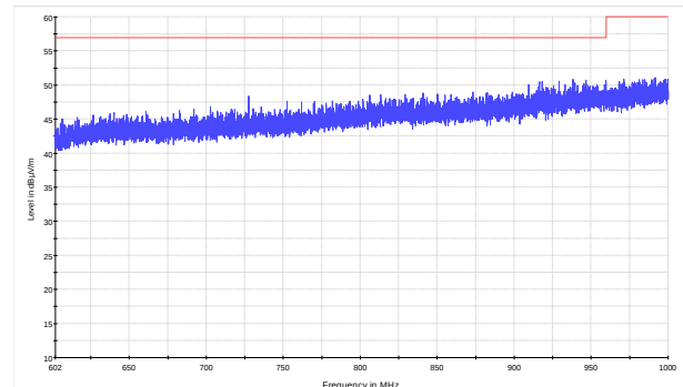
Figure 8.9-4: Radiated spurious emissions within 602–1000 MHz for mid channel for LPDA antenna (BTS)
