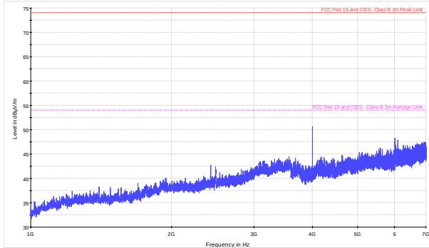
Figure 8.9-37: Radiated spurious emissions within 1–7 GHz for low channel for LPDA antenna (CPE)
