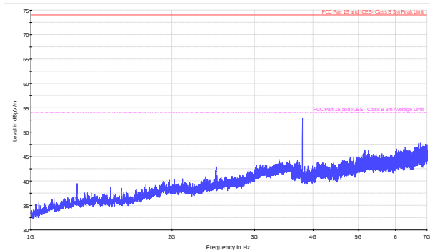
Figure 8.9-41: Radiated spurious emissions within 1–7 GHz for mid channel for Panel antenna (CPE)
