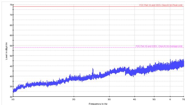
Figure 8.9-33: Radiated spurious emissions within 1–7 GHz for high channel for LPDA antenna (BTS)
