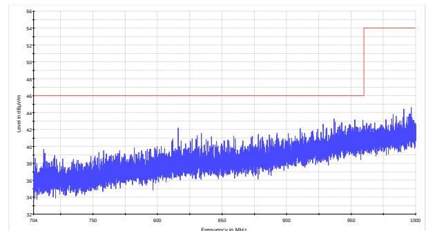
Figure 8.9-30: Radiated spurious emissions within 704–1000 MHz for high channel for Omnidirectional antenna (CPE)
