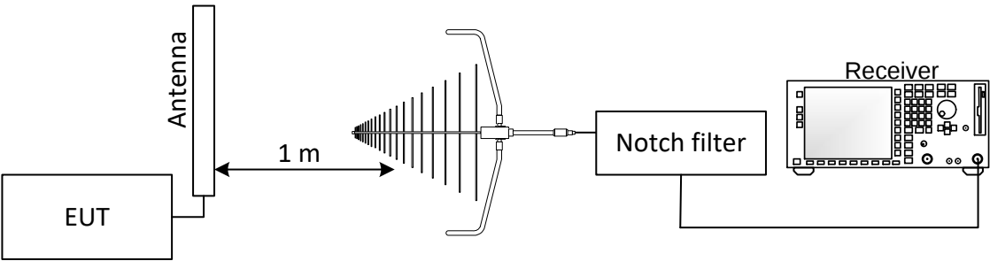
Figure 8.10-1: Setup diagram for 602–620 MHz radiated emissions measurements
