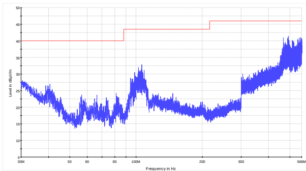
Figure 8.9-21: Radiated spurious emissions within 30–566 MHz for mid channel for Panel antenna (CPE)
