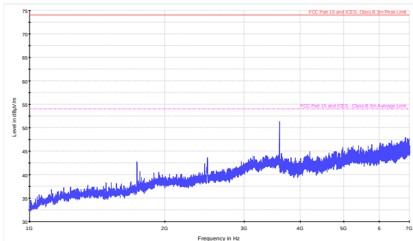
Figure 8.9-45: Radiated spurious emissions within 1–7 GHz for high channel for Omnidirectional antenna (CPE)
