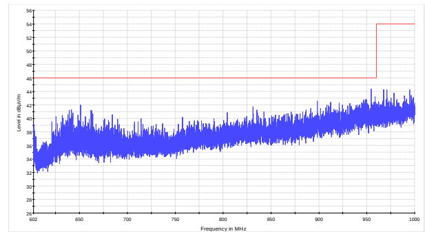
Figure 8.9-22: Radiated spurious emissions within 602–1000 MHz for mid channel for Panel antenna (B CPE TS)
