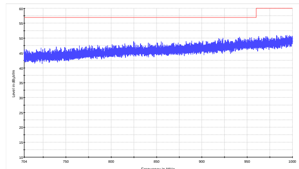
Figure 8.9-6: Radiated spurious emissions within 704–1000 MHz for high channel for LPDA antenna (BTS)
