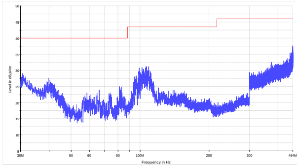
Figure 8.9-19: Radiated spurious emissions within 30–464 MHz for low channel for Panel antenna (CPE)
