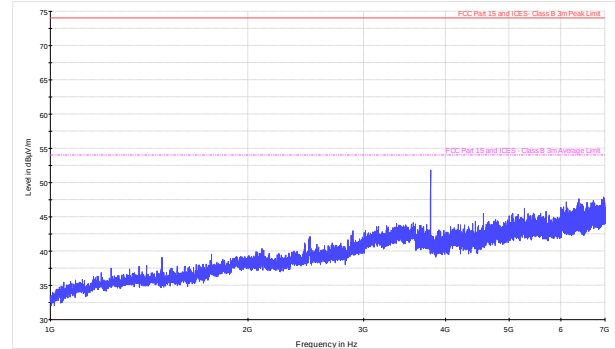
Figure 8.9-38: Radiated spurious emissions within 1–7 GHz for mid channel for LPDA antenna (CPE)
