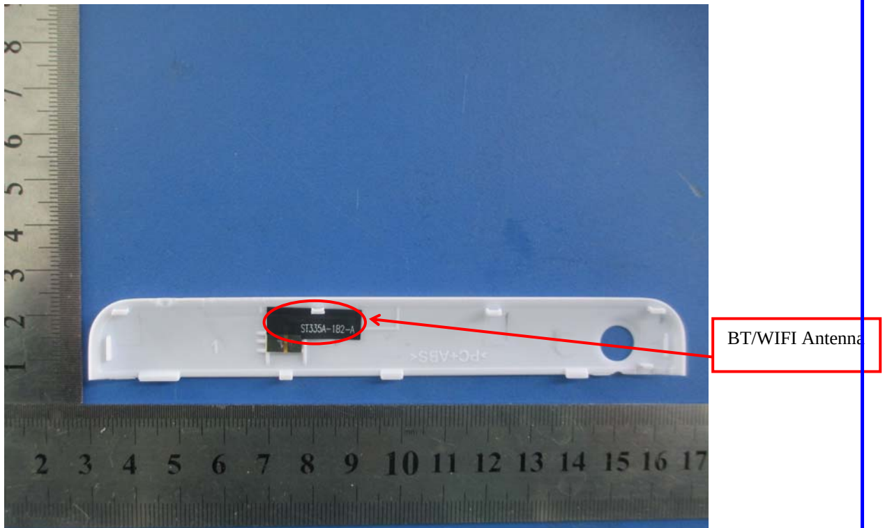
BT&WIFI Antenna – Front View
