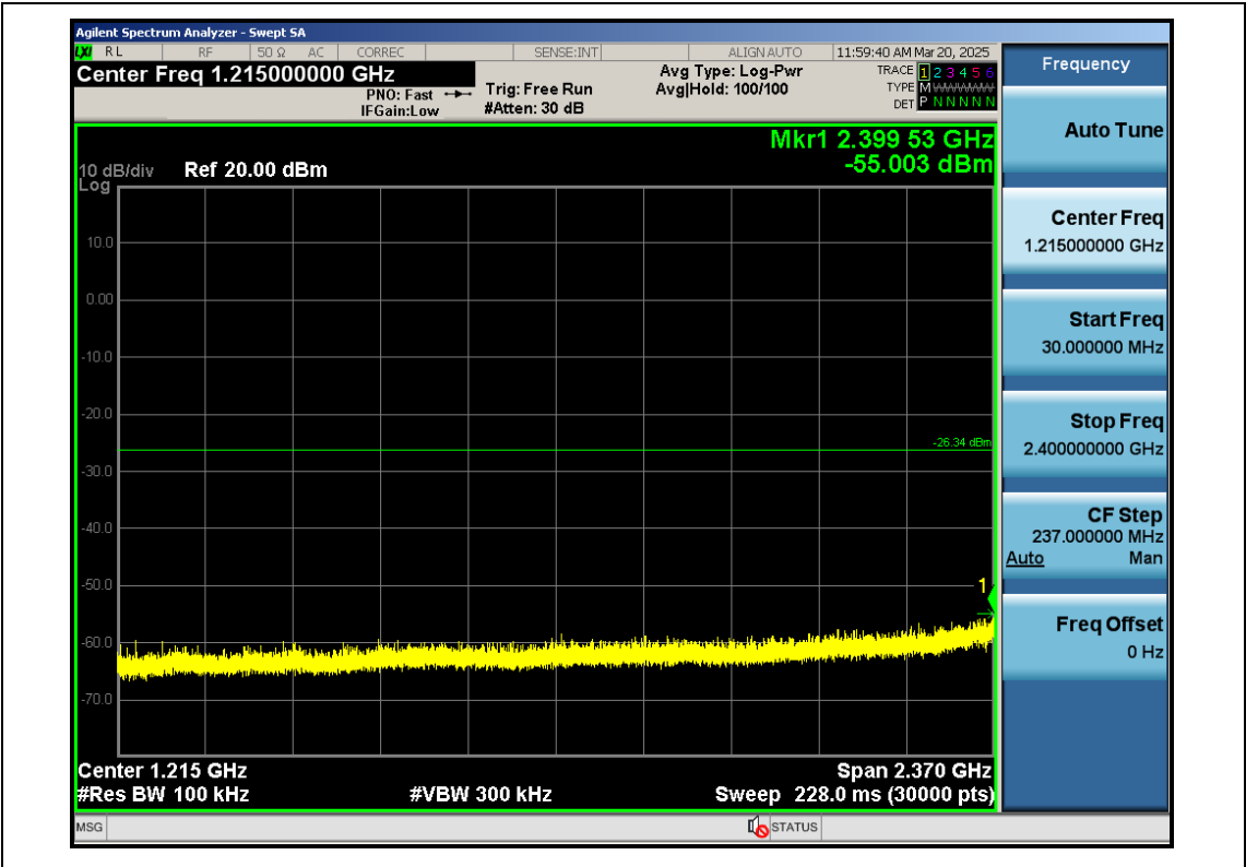
11N40SISO-Ant1-2437-30~2400-PASS
