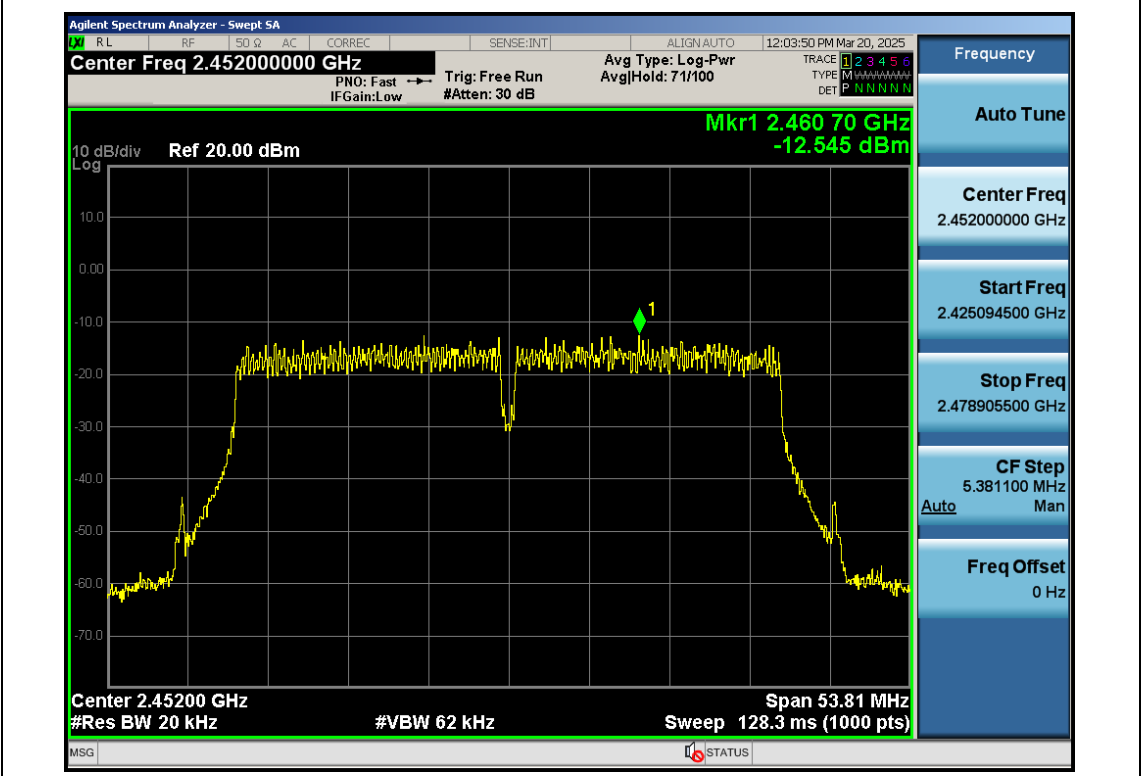
11N40SISO-Ant1-2452-PASS
