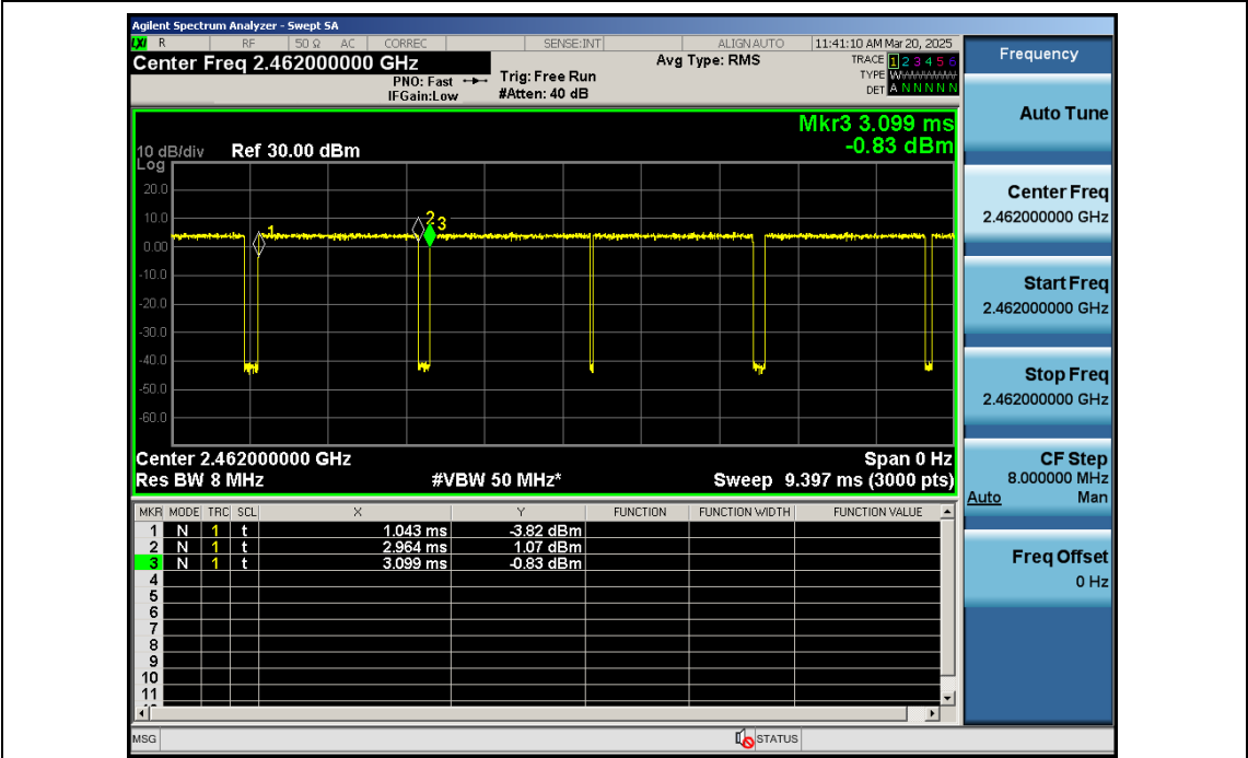
NTNV-11N20SISO-Ant1-2462
