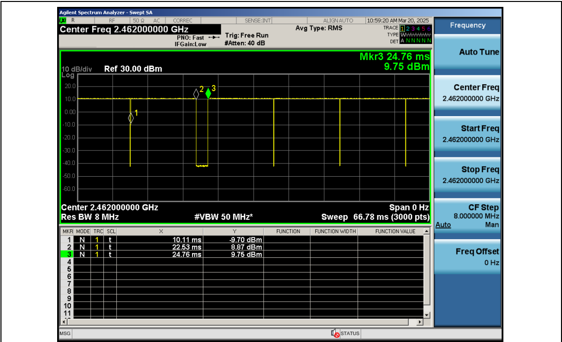
NTNV-11B-Ant1-2462
