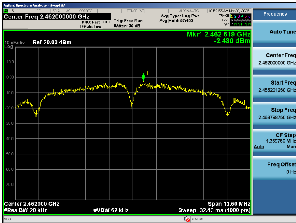
11B-Ant1-2462-PASS
