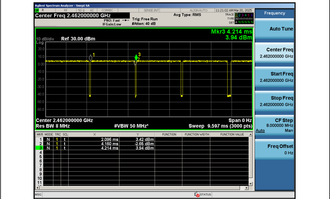
NTNV-11G-Ant1-2462
