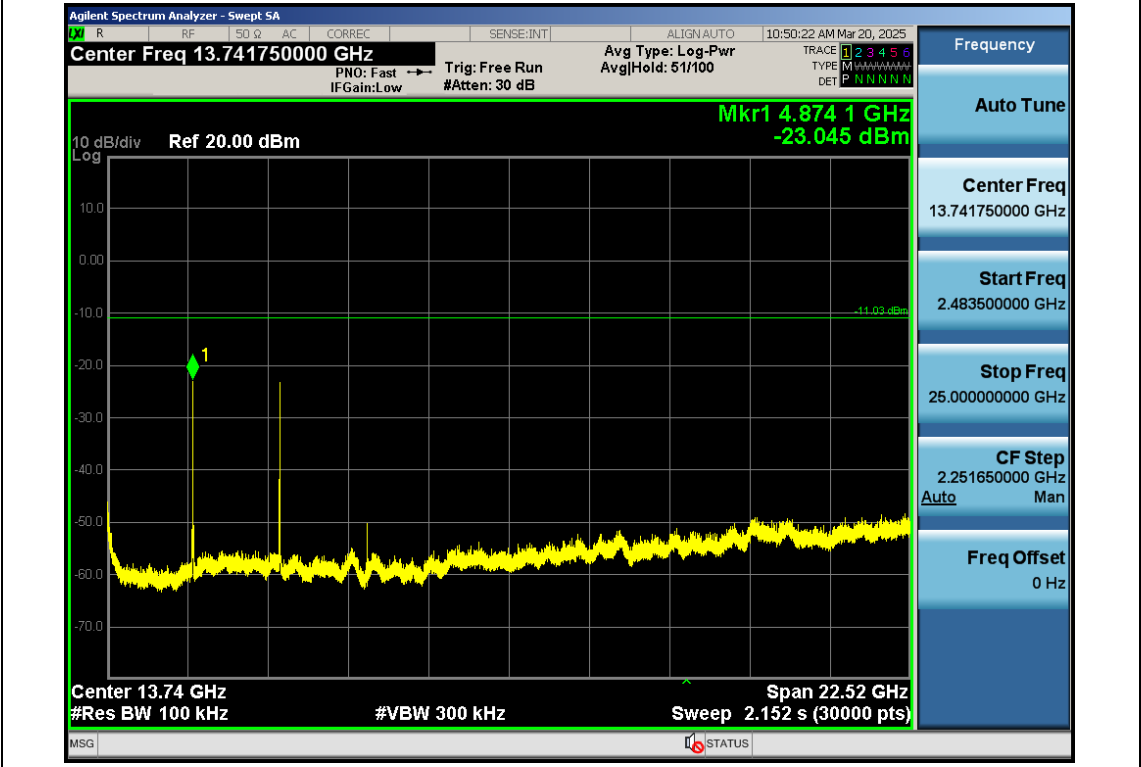
11B-Ant1-2437-2483.5~25000-PASS
