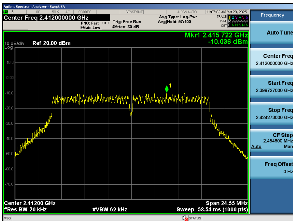
11G-Ant1-2412-PASS
