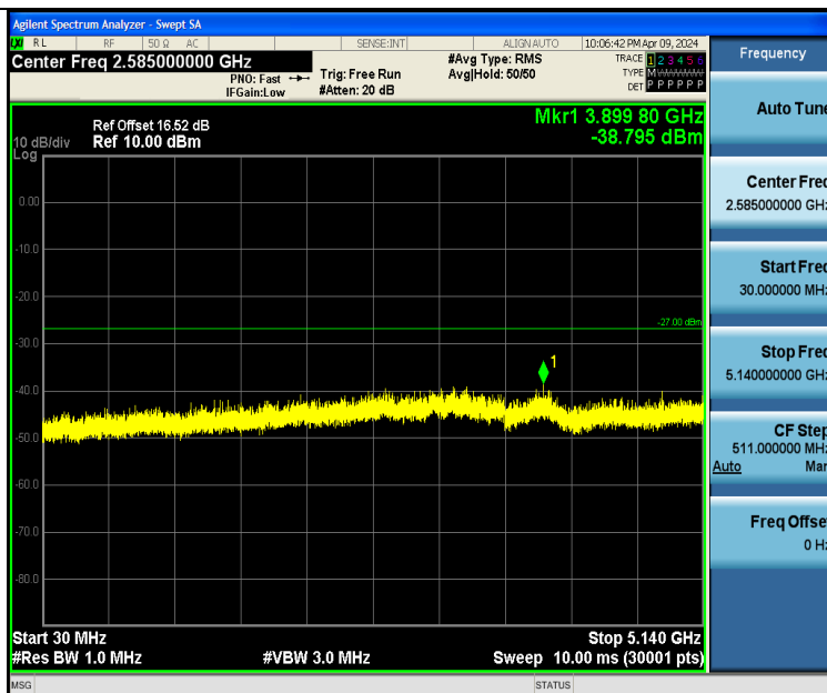
11AC20SISO-Ant2-5240-30~5140-PASS
