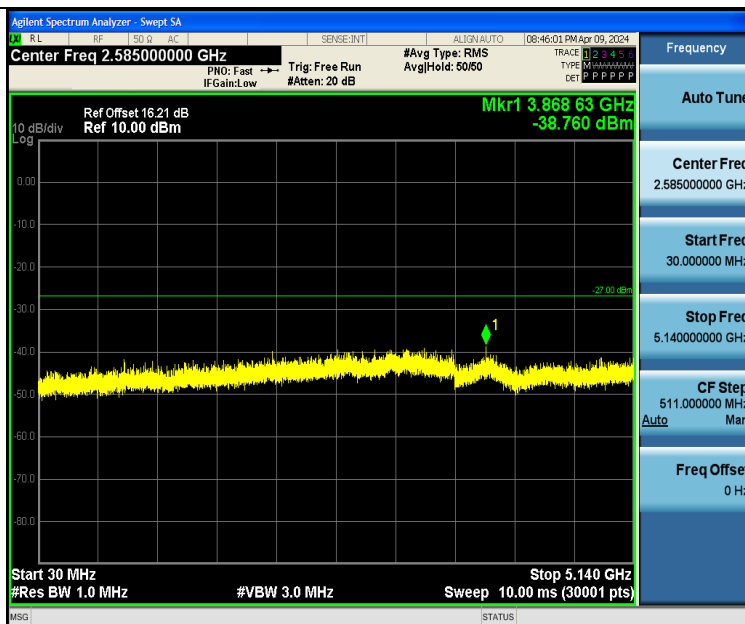
11A-Ant2-5180-30~5140-PASS
