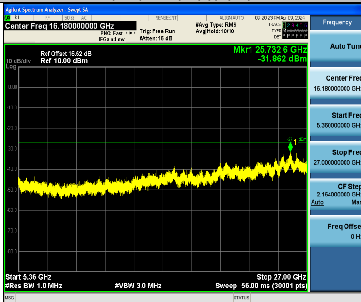
11N20SISO-Ant2-5240-5360~27000-PASS
