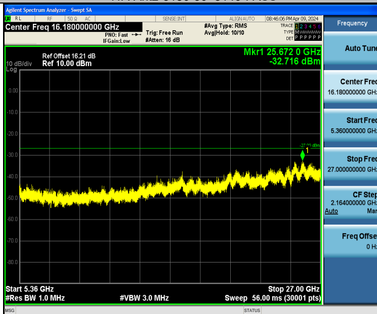
11A-Ant2-5180-5360~27000-PASS
