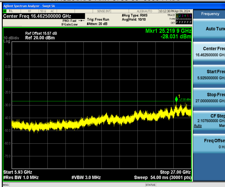
11AC20SISO-Ant1-5785-5925~27000-PASS
