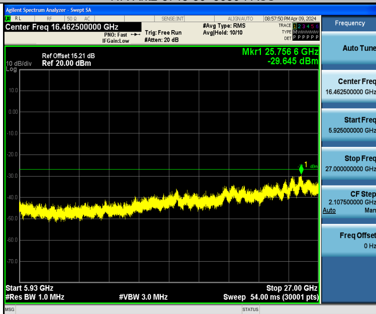
11A-Ant2-5745-5925~27000-PASS
