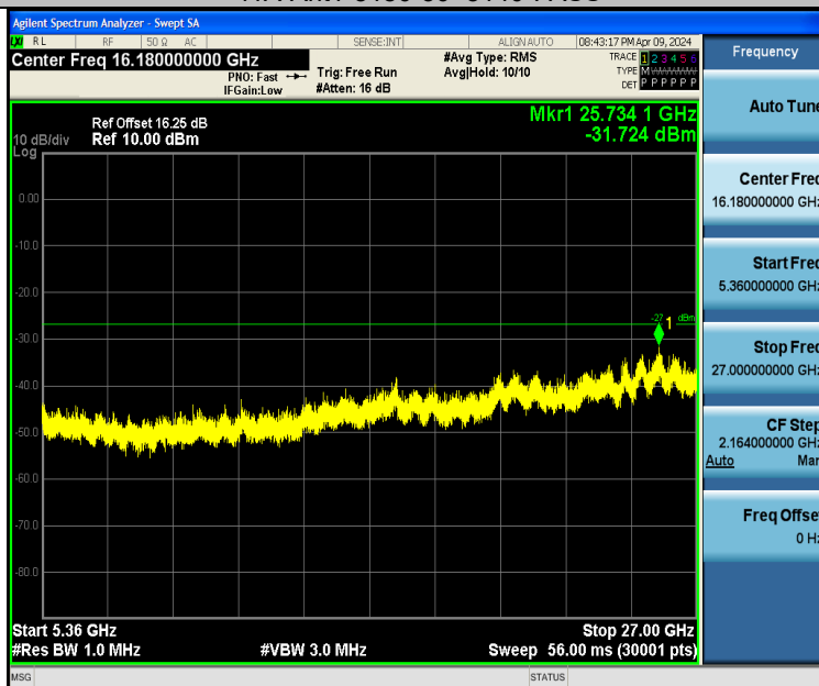
11A-Ant1-5180-5360~27000-PASS
