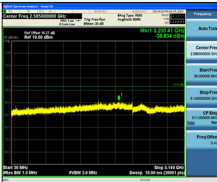
11A-Ant2-5200-30~5140-PASS
