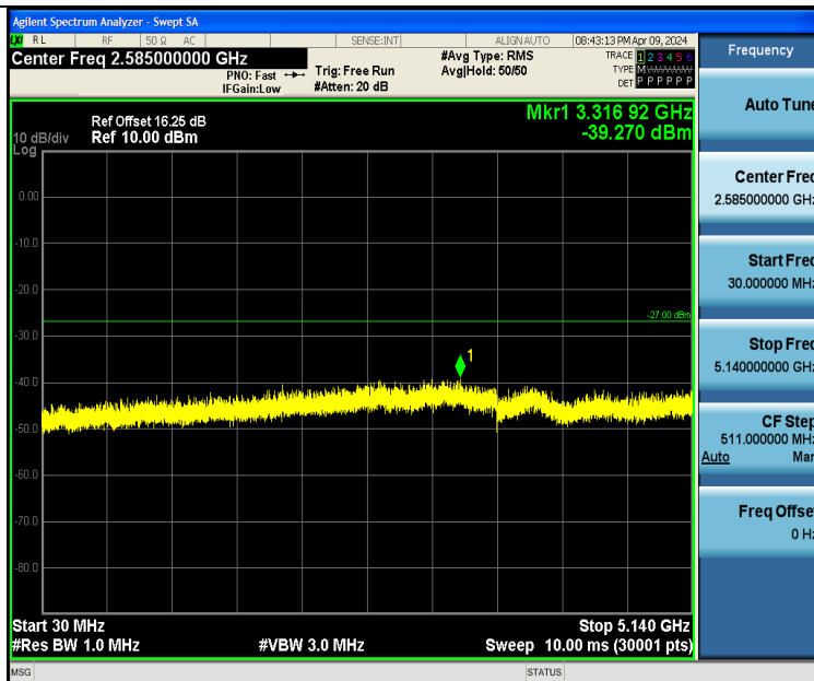
11A-Ant1-5180-30~5140-PASS
