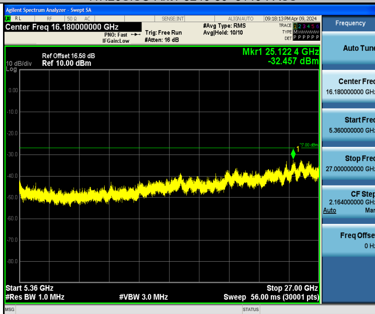
11N20SISO-Ant1-5240-5360~27000-PASS
