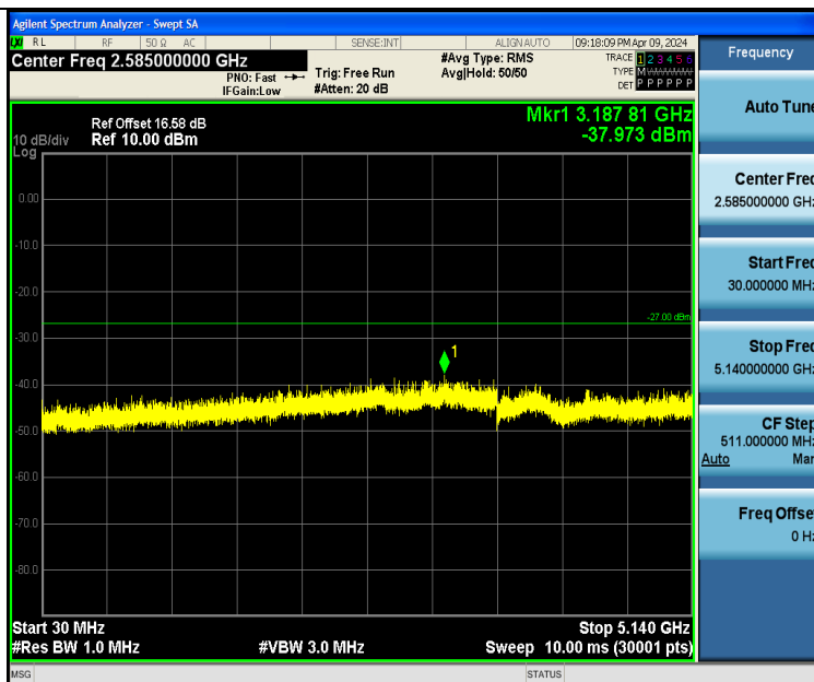
11N20SISO-Ant1-5240-30~5140-PASS
